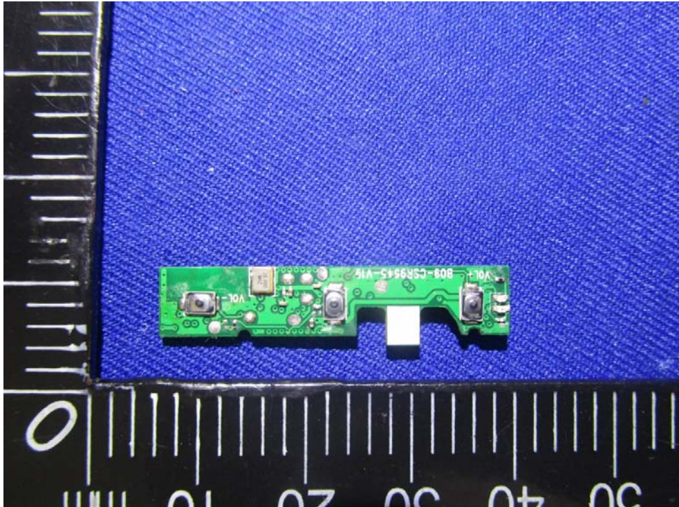
EUT – Audio Module Bottom View
