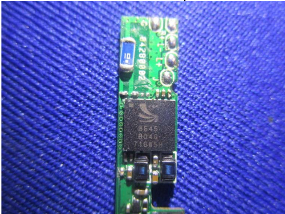
EUT – Audio Module RF Chip View
