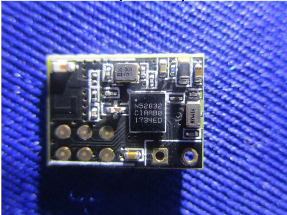
EUT – Step Module RF Chip View
