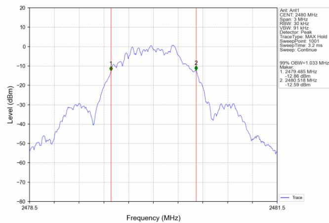
1M_HCH_2480MHz_Ant1_NTNV
