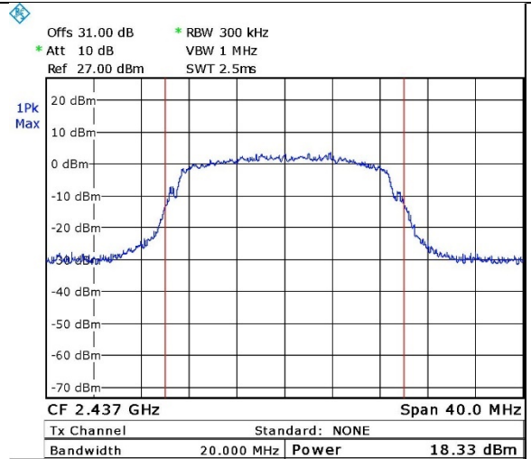
Figure 47. 2437.0 MHz, Wi-fi/n(65Mbit/s)
