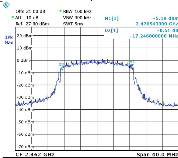
Figure 31. 2462.0 MHz, Wi-fi/n(65Mbit/s)
