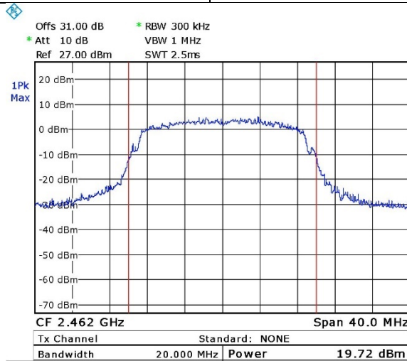
Figure 48. 2462.0 MHz, Wi-fi/n(65Mbit/s)
