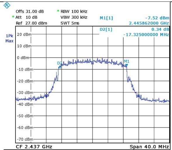
Figure 30. 2437.0 MHz, Wi-fi/n(65Mbit/s)
