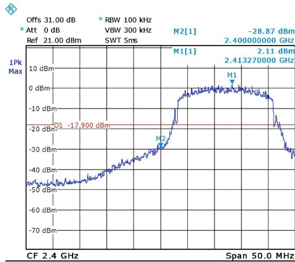
Figure 59 Band Edge Low, Wi-fi/n(65Mbit/s)
