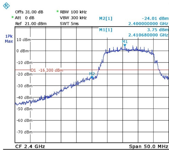
Figure 53 Band Edge Low, Wi-fi/g(6Mbit/s)
