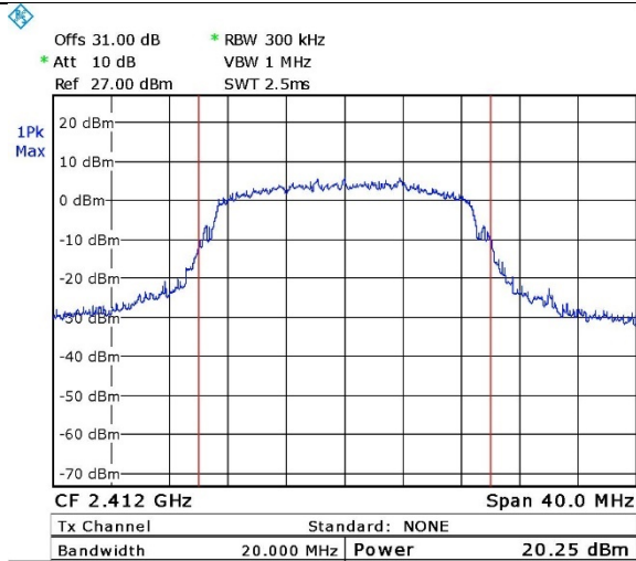
Figure 46. 2412.0 MHz, Wi-fi/n(65Mbit/s)
