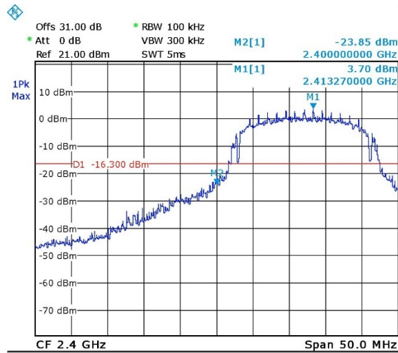
Figure 57 Band Edge Low, Wi-fi/n(6.5Mbit/s)
