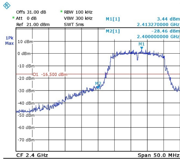
Figure 55 Band Edge Low, Wi-fi/g(54Mbit/s)
