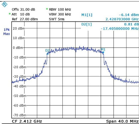
Figure 29. 2412.0 MHz, Wi-fi/n(65Mbit/s)
