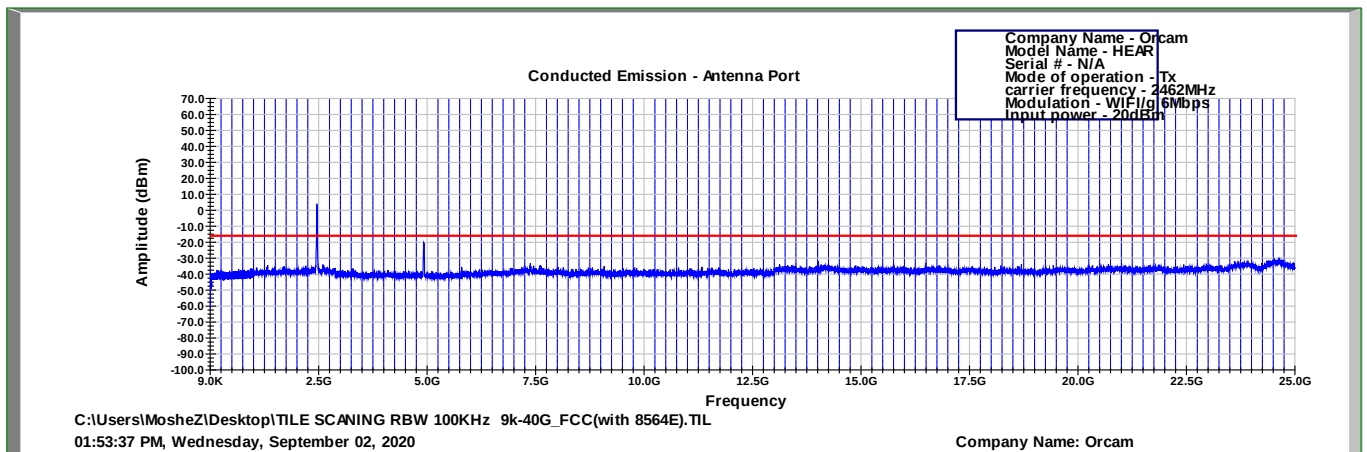
Figure 101 2462.0 MHz, WI-FI/g(6Mbit/s)
