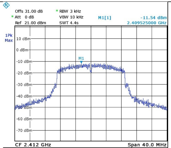
Figure 70. 2412.0 MHz, Wi-fi/n(6.5Mbit/s)
