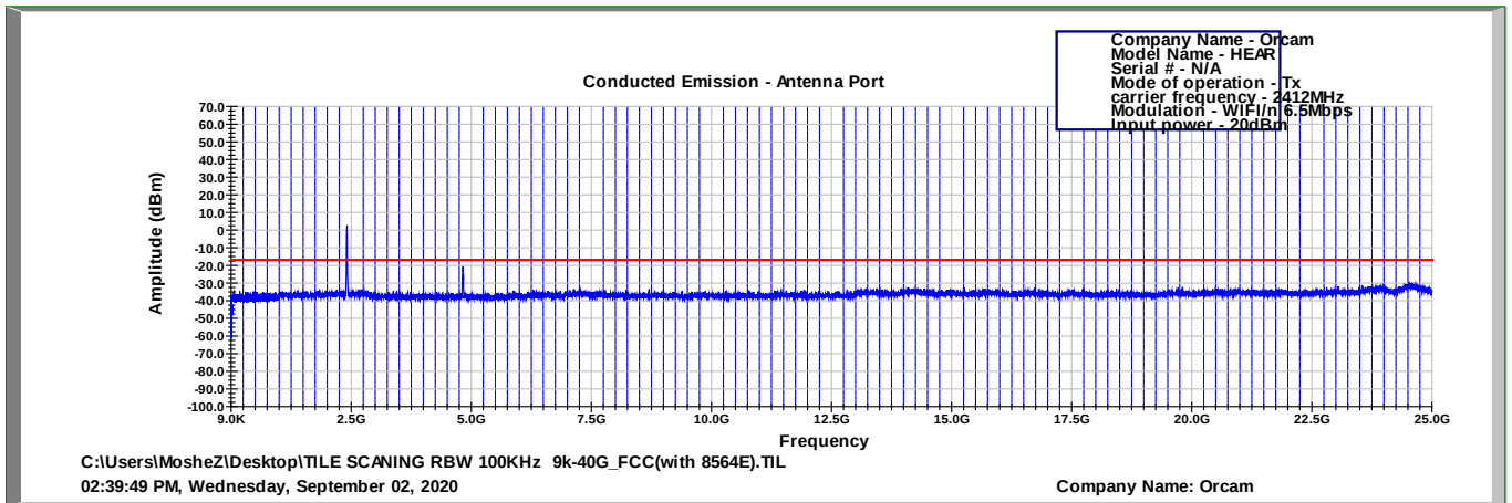
Figure 105 2412.0 MHz, WI-FI/n(6.5Mbit/s)
