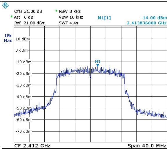
Figure 75. 2412.0 MHz, Wi-fi/n(65Mbit/s)
