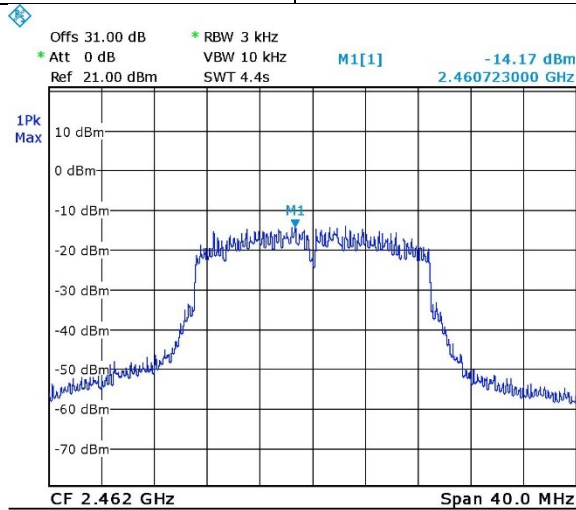
Figure 77. 2462.0 MHz, Wi-fi/n(65Mbit/s)
