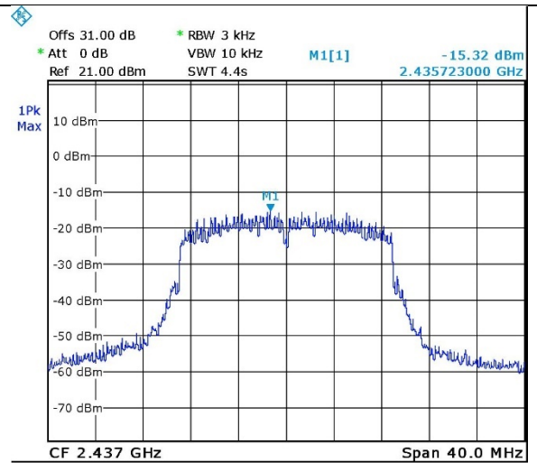
Figure 76. 2437.0 MHz, Wi-fi/n(65Mbit/s)
