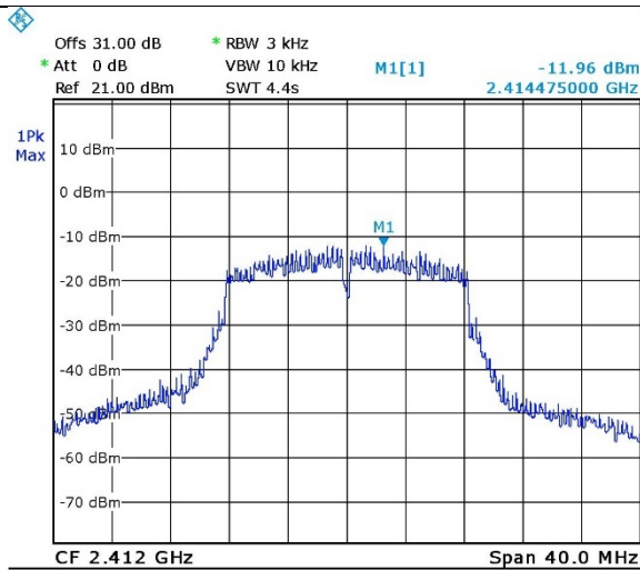
Figure 69. 2412.0 MHz, Wi-fi/g(54Mbit/s)
