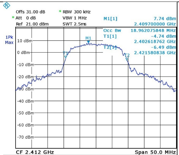
Figure 81. 2412.0 MHz, Wi-fi/g(6Mbit/s)
