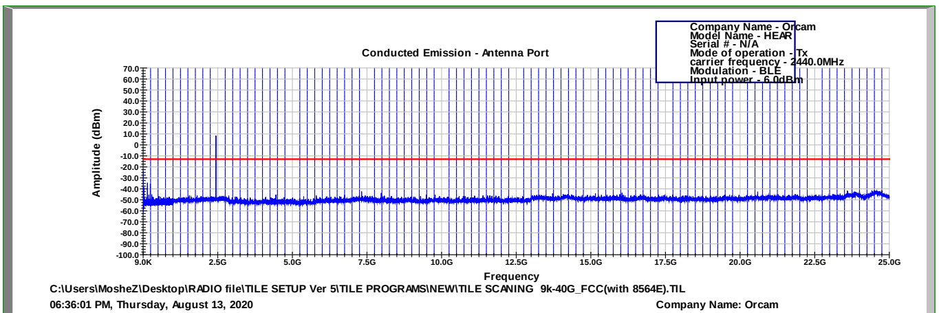
Figure 97 2440.0 MHz, BLE
