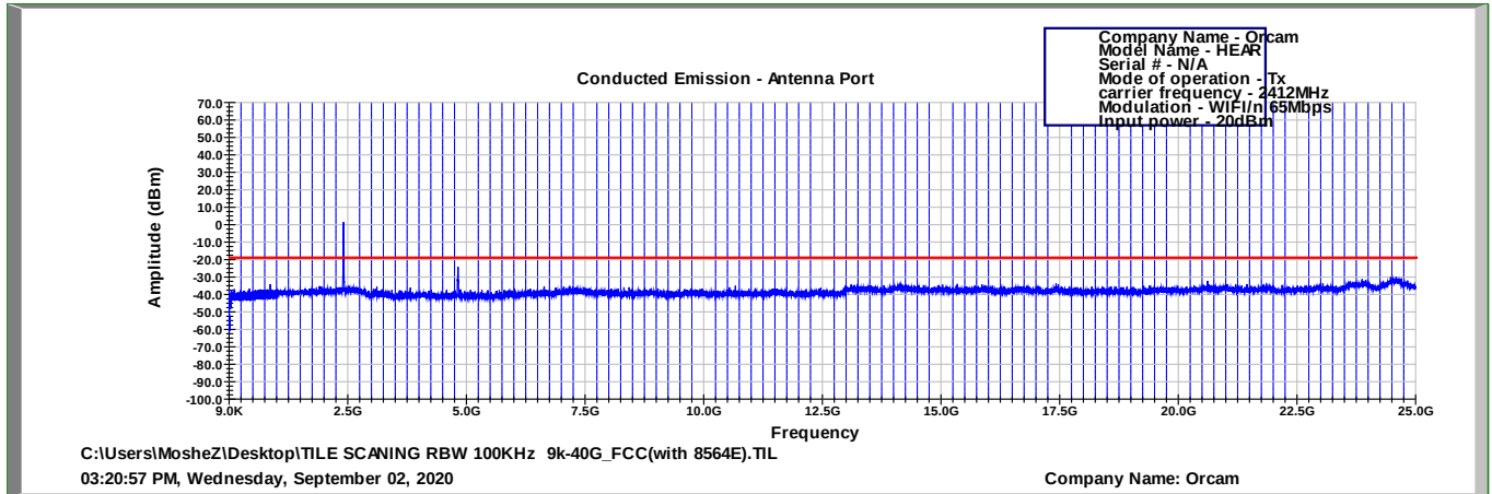
Figure 108 2412.0 MHz, WI-FI/n(65Mbit/s)
