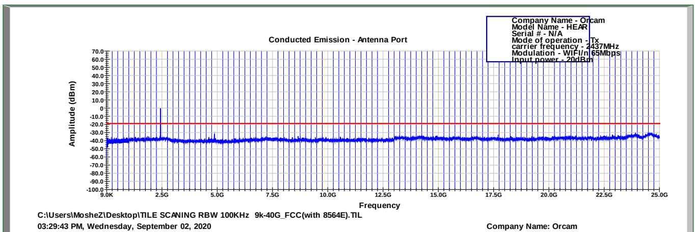
Figure 109 2437.0 MHz, WI-FI/n(65Mbit/s)
