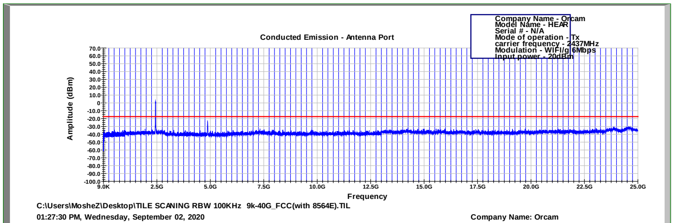
Figure 100 2437.0 MHz, WI-FI/g(6Mbit/s)
