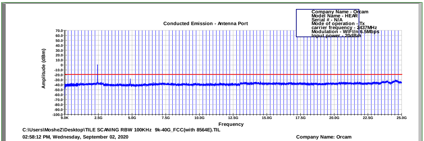
Figure 106 2437.0 MHz, WI-FI/n(6.5Mbit/s)
