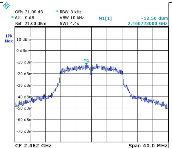
Figure 68. 2462.0 MHz, Wi-fi/g(6Mbit/s)
