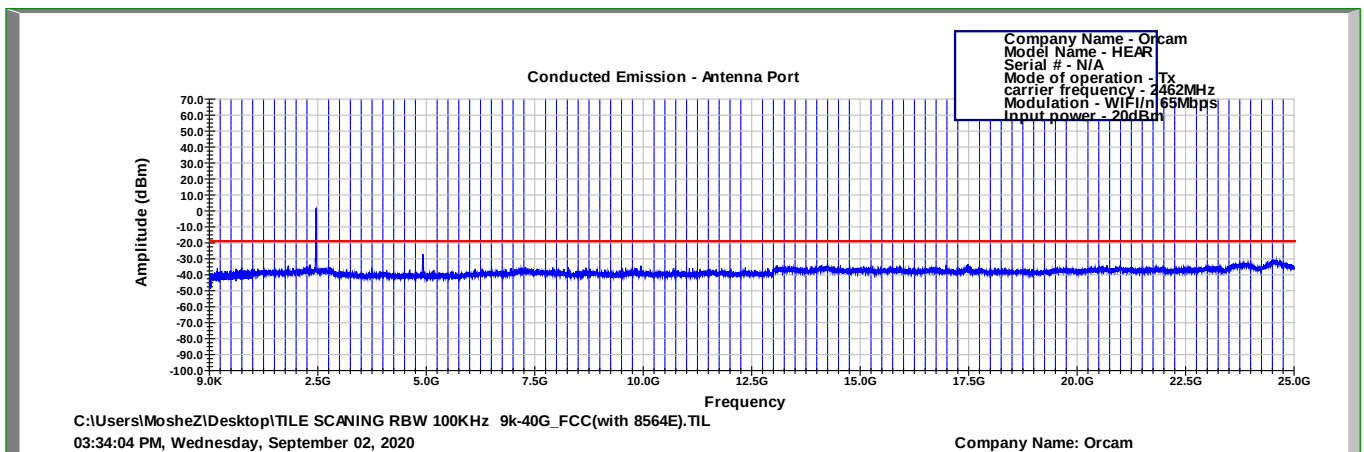
Figure 110 2462.0 MHz, WI-FI/n(65Mbit/s)
