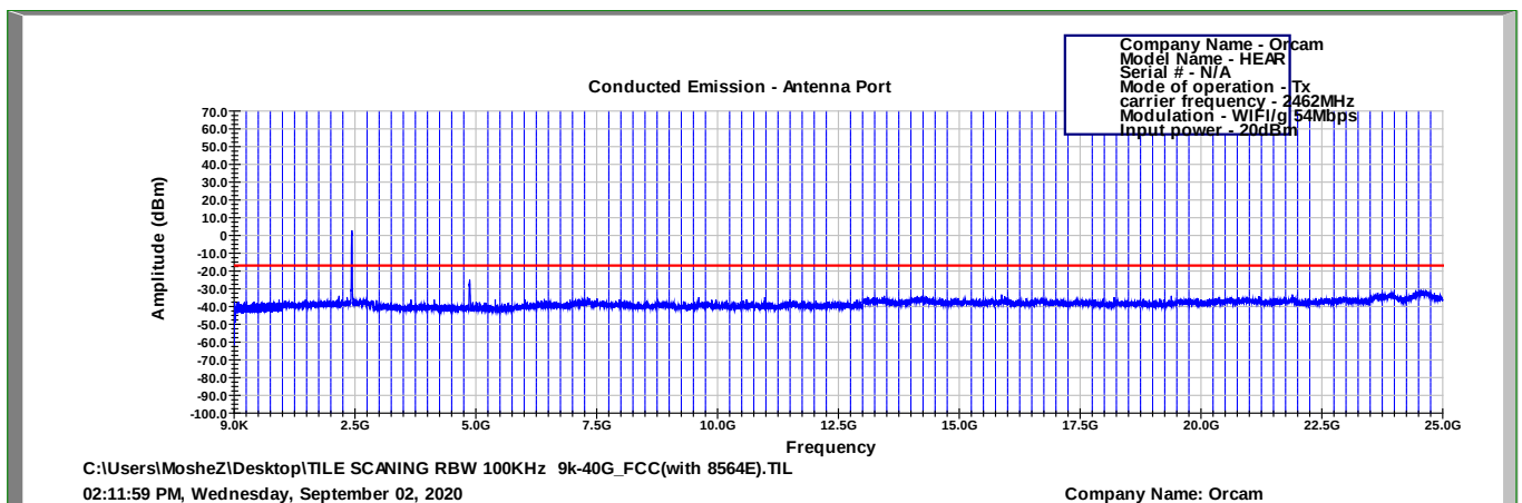
Figure 104 2462.0 MHz, WI-FI/g(54Mbit/s)
