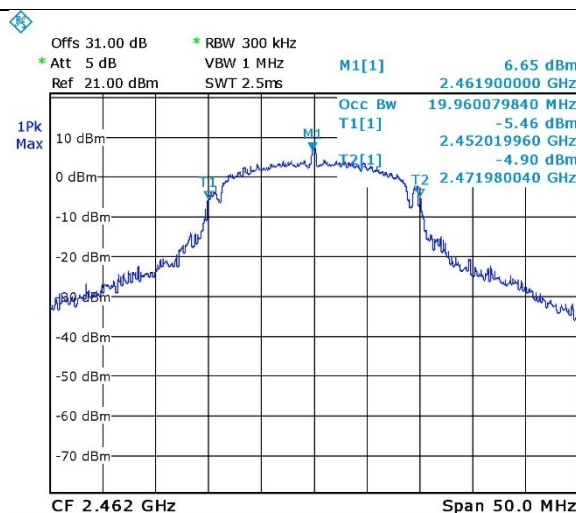
Figure 91. 2462.0 MHz, Wi-fi/n(6.5Mbit/s)
