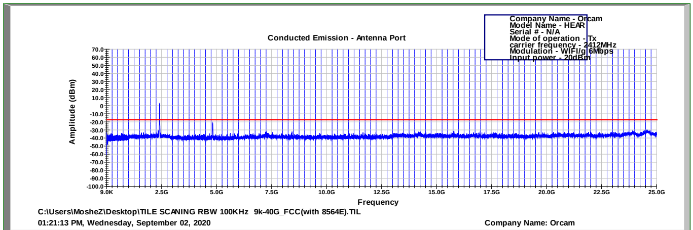
Figure 99 2412.0 MHz, WI-FI/g(6Mbit/s)
