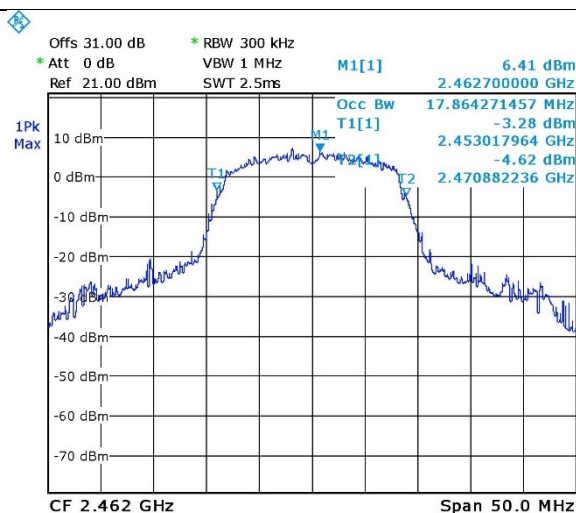
Figure 90. 2462.0 MHz, Wi-fi/g(54Mbit/s)
