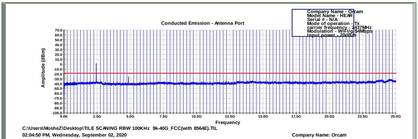
Figure 103 2437.0 MHz, WI-FI/g(54Mbit/s)
