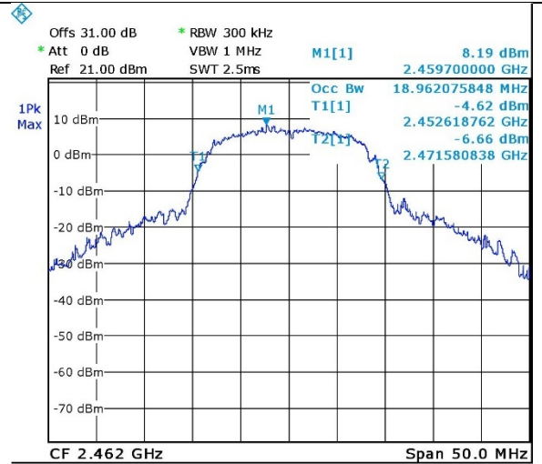
Figure 85. 2462.0 MHz, Wi-fi/g(6Mbit/s)
