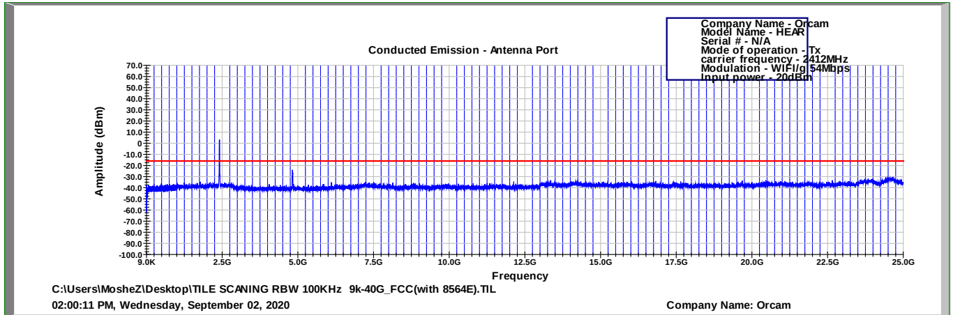
Figure 102 2412.0 MHz, WI-FI/g(54Mbit/s)
