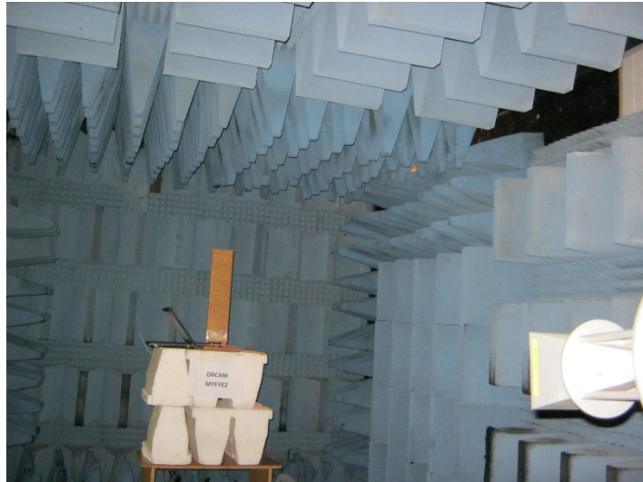
Radiated Emission Test, 18-26.5GHz
