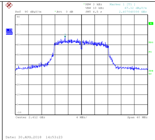
Figure 83 2412.0 MHz, Wi-fi/g(6Mbit/s)
