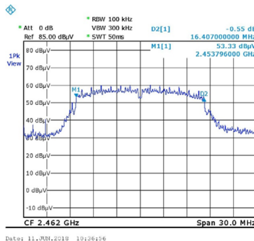
Figure 29. 2462.0 MHz, Wi-fi/g(54Mbit/s)
