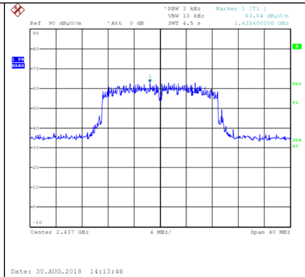
Figure 91. 2437.0 MHz, Wi-fi/n(6.5Mbit/s)
