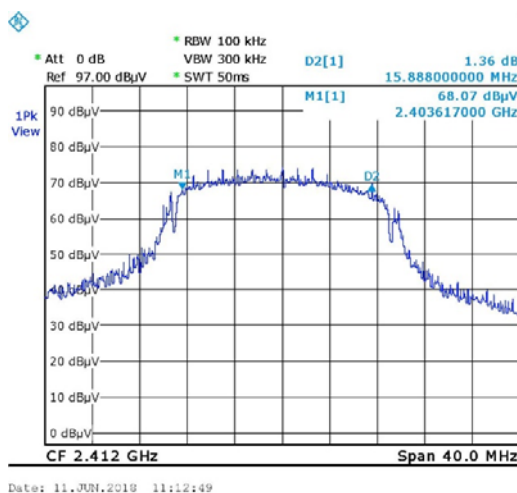
Figure 30. 2412.0 MHz, Wi-fi/n(6.5Mbit/s)
