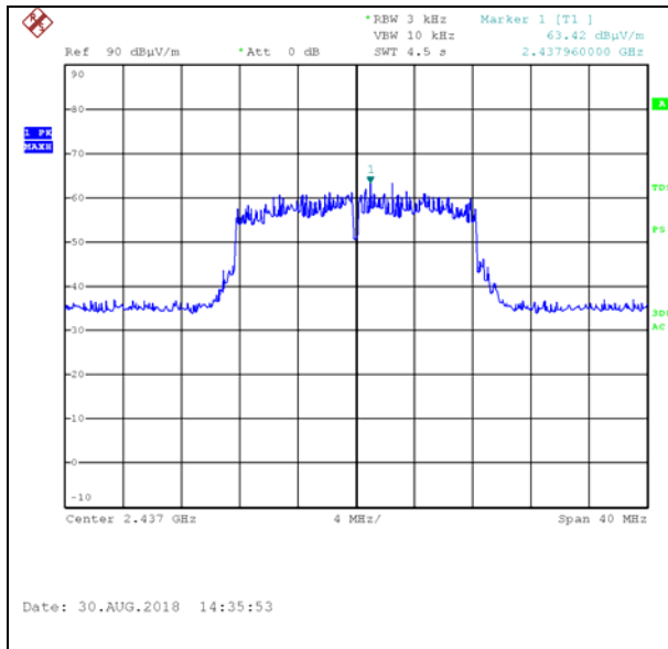
Figure 90. 2437.0 MHz, Wi-fi/g(54Mbit/s)
