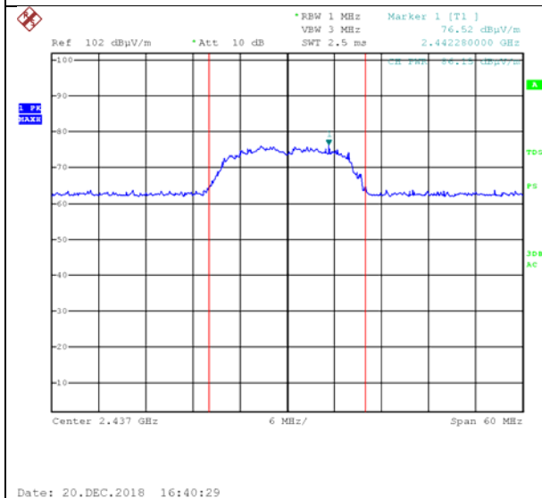
Figure 52. 2437.0 MHz, Wi-fi/g(54Mbit/s), Vertical
