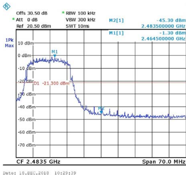
Figure 79 Band Edge High, Wi-fi/n(65Mbit/s)
