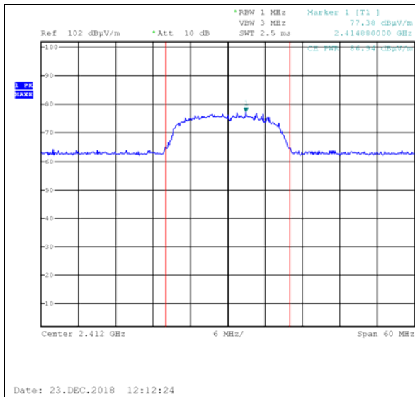
Figure 62. 2412.0 MHz, Wi-fi/n(65Mbit/s), Vertical
