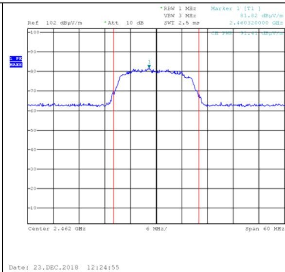
Figure 67. 2462.0 MHz, Wi-fi/n(65Mbit/s), Horizontal
