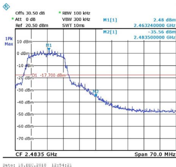
Figure 73 Band Edge High, Wi-fi/g(6Mbit/s)
