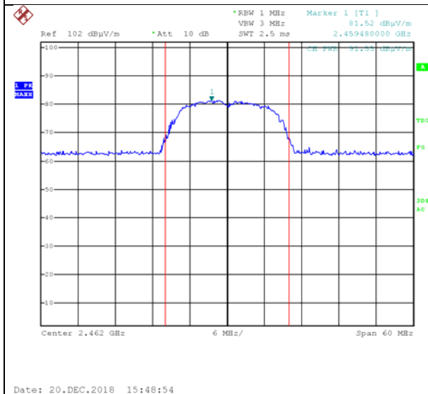
Figure 48. 2462.0 MHz, Wi-fi/g(6Mbit/s), Vertical
