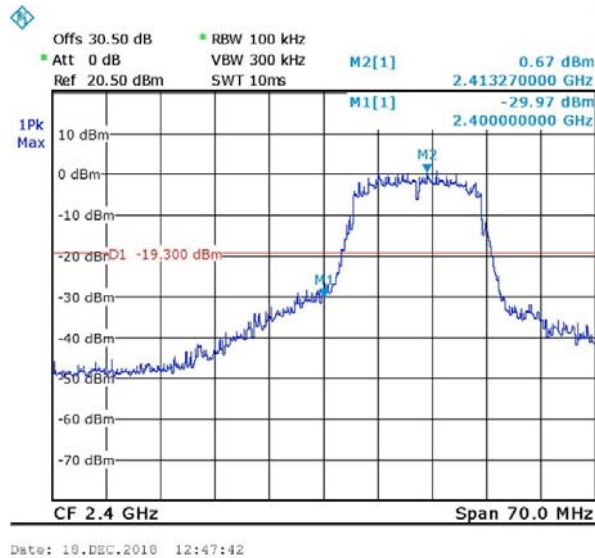
Figure 74 Band Edge Low, Wi-fi/g(54Mbit/s)
