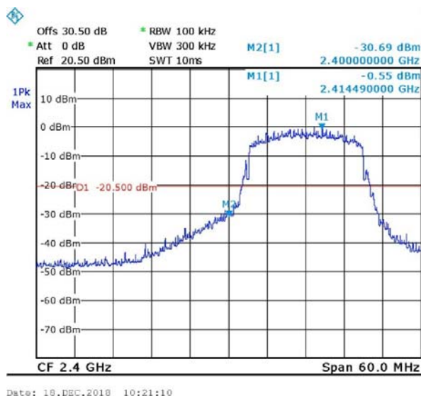
Figure 78 Band Edge Low, Wi-fi/n(65Mbit/s)
