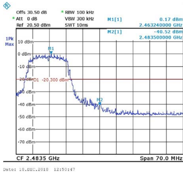
Figure 75 Band Edge High, Wi-fi/g(54Mbit/s)
