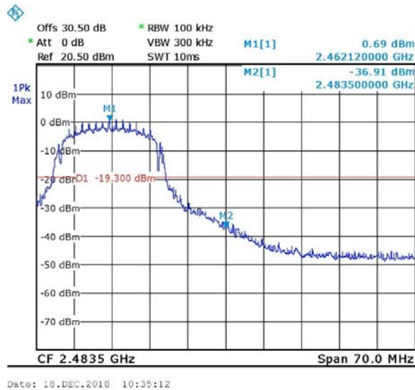
Figure 77 Band Edge High, Wi-fi/n(6.5Mbit/s)
