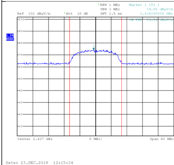
Figure 64. 2437.0 MHz, Wi-fi/n(65Mbit/s), Vertical
