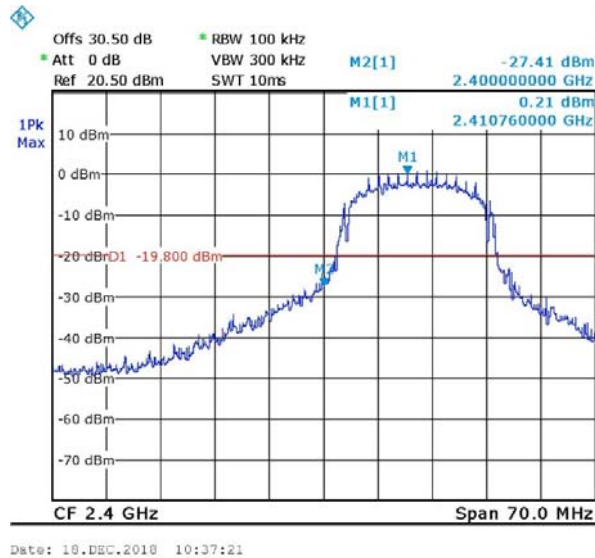
Figure 76 Band Edge Low, Wi-fi/n(6.5Mbit/s)
