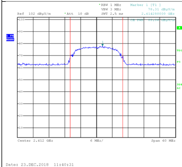
Figure 56. 2412.0 MHz, Wi-fi/n(6.5Mbit/s), Vertical
