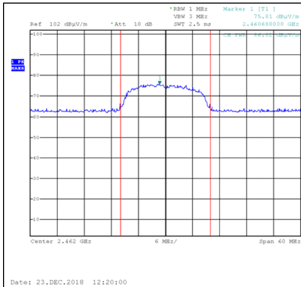
Figure 66. 2462.0 MHz, Wi-fi/n(65Mbit/s), Vertical
