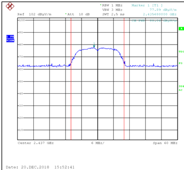
Figure 46. 2437.0 MHz, Wi-fi/g(6Mbit/s), Vertical
