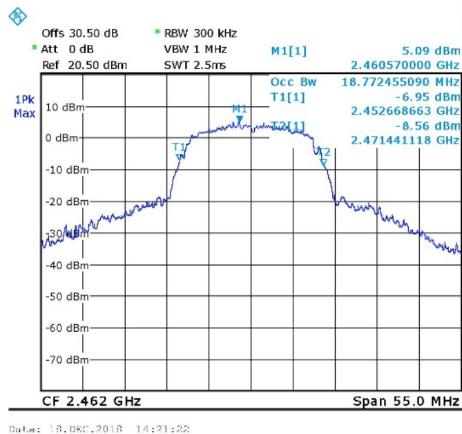
Figure 104. 2462.0 MHz, Wi-fi/g(6Mbit/s)
