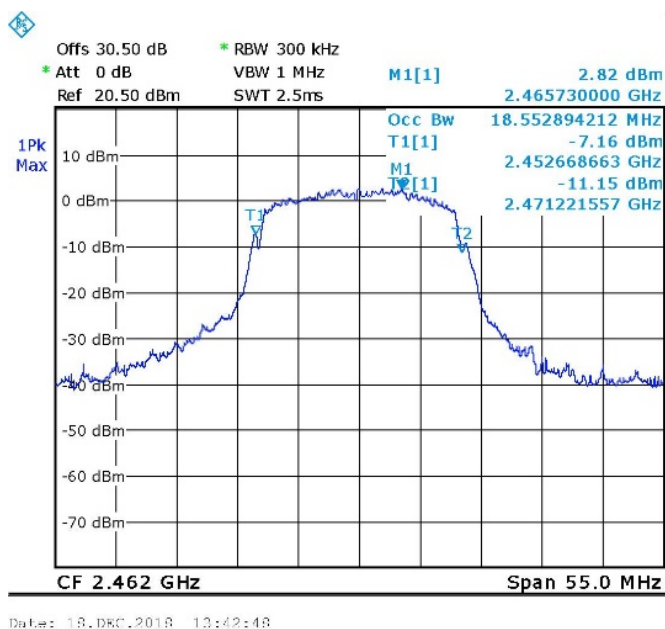
Figure 113. 2462.0 MHz, Wi-fi/n(65Mbit/s)
