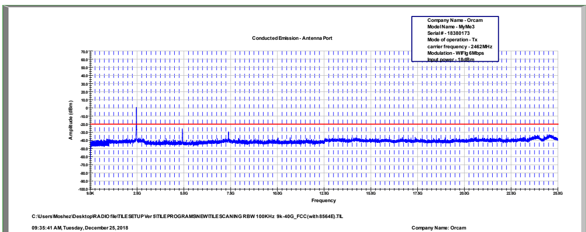
Figure 120 2462.0 MHz, WI-FI/g(6Mbit/s)
