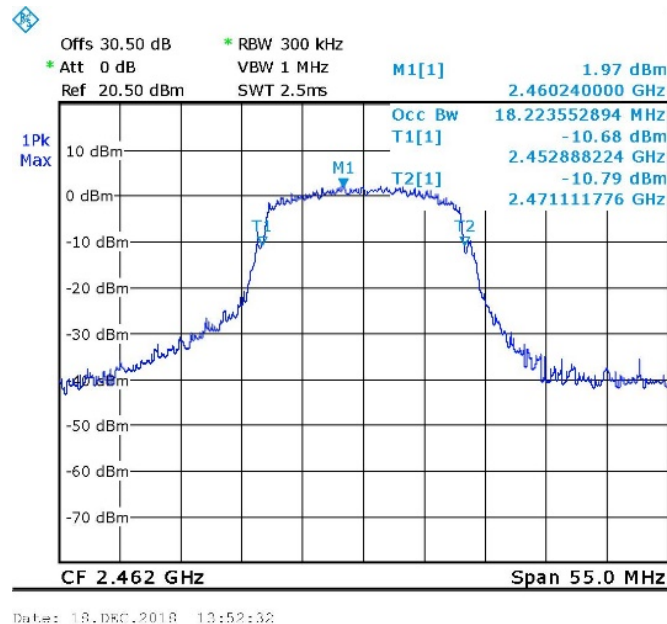
Figure 110. 2462.0 MHz, Wi-fi/n(6.5Mbit/s)
