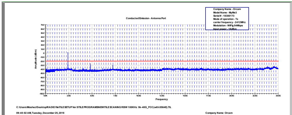
Figure 121 2412.0 MHz, WI-FI/g(54Mbit/s)
