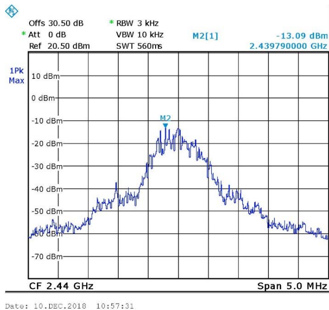
Figure 83. 2440.0 MHz, BLE
