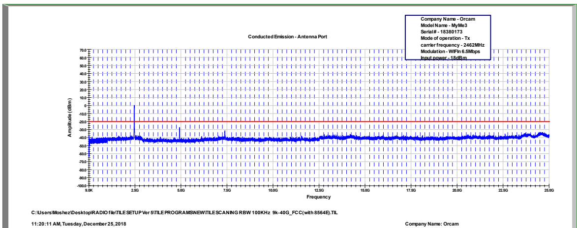
Figure 126 2462.0 MHz, WI-FI/n(6.5Mbit/s)
