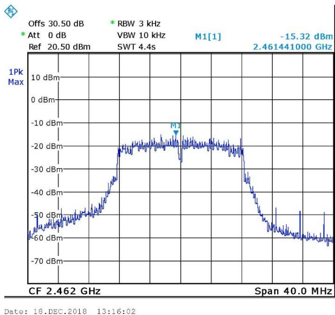
Figure 90. 2462.0 MHz, Wi-fi/g(54Mbit/s)
