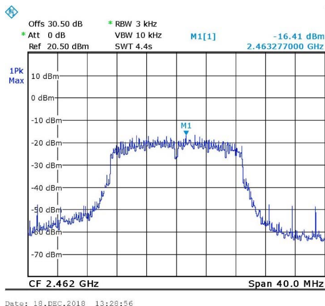
Figure 96. 2462.0 MHz, Wi-fi/n(65Mbit/s)
