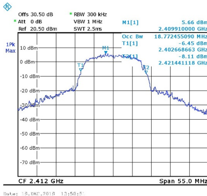
Figure 102. 2412.0 MHz, Wi-fi/g(6Mbit/s)
