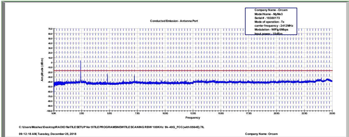
Figure 118 2412.0 MHz, WI-FI/g(6Mbit/s)
