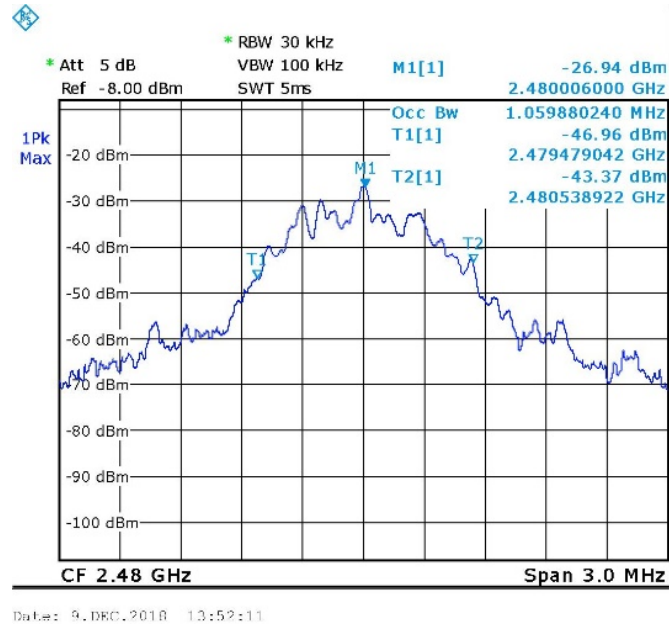
Figure 101. 2480.0 MHz, BLE
