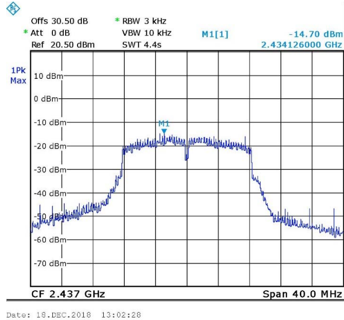
Figure 86. 2437.0 MHz, Wi-fi/g(6Mbit/s)
