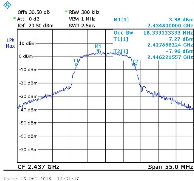
Figure 103. 2437.0 MHz, Wi-fi/g(6Mbit/s)
