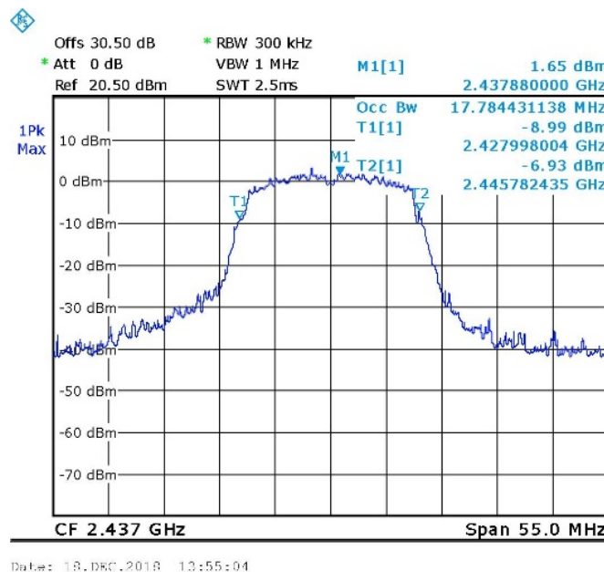
Figure 106. 2437.0 MHz, Wi-fi/g(54Mbit/s)
