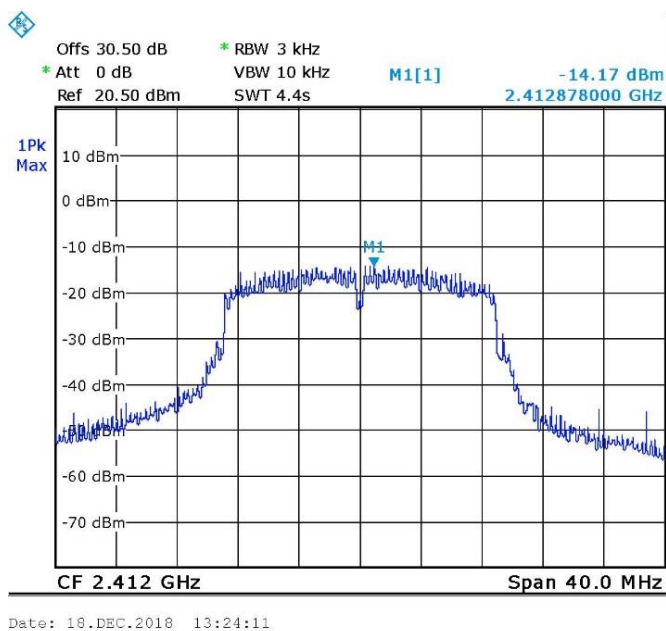
Figure 91. 2412.0 MHz, Wi-fi/n(6.5Mbit/s)
