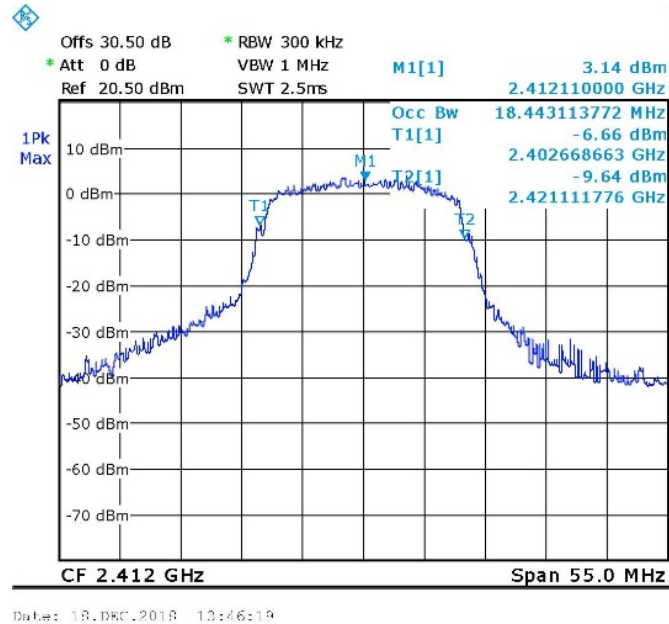
Figure 111. 2412.0 MHz, Wi-fi/n(65Mbit/s)
