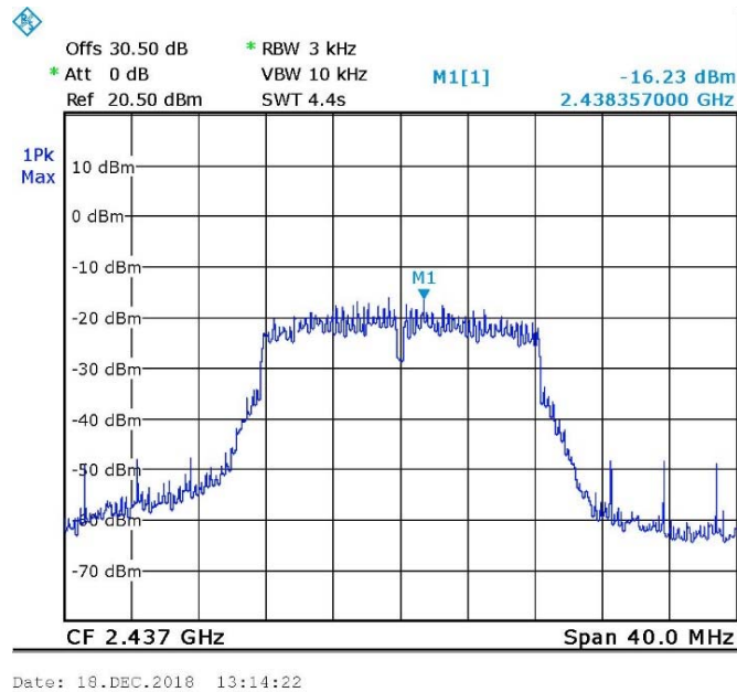
Figure 89. 2437.0 MHz, Wi-fi/g(54Mbit/s)
