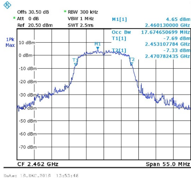
Figure 107. 2462.0 MHz, Wi-fi/g(54Mbit/s)
