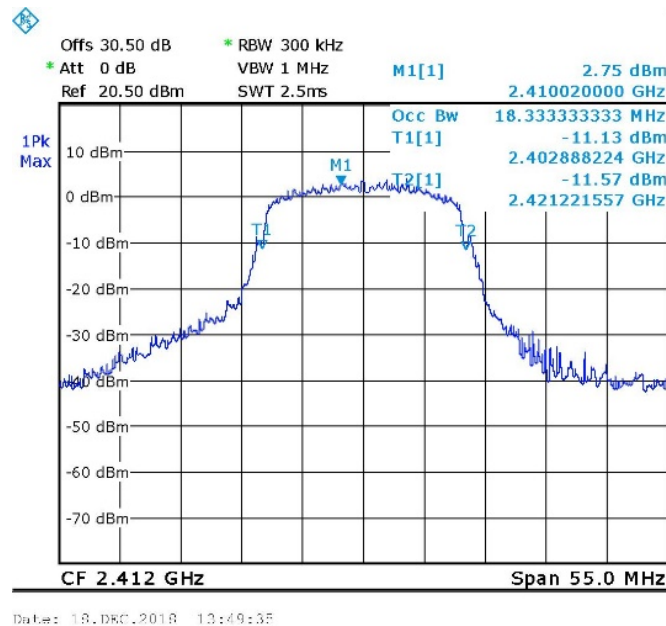
Figure 108. 2412.0 MHz, Wi-fi/n(6.5Mbit/s)
