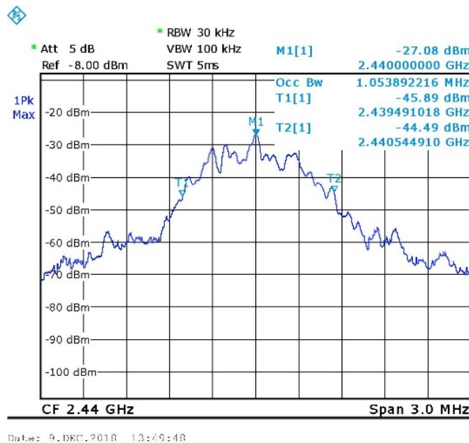
Figure 100. 2440.0 MHz, BLE
