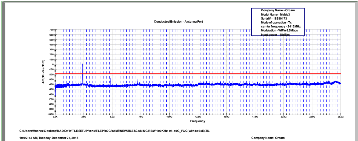
Figure 124 2412.0 MHz, WI-FI/n(6.5Mbit/s)
