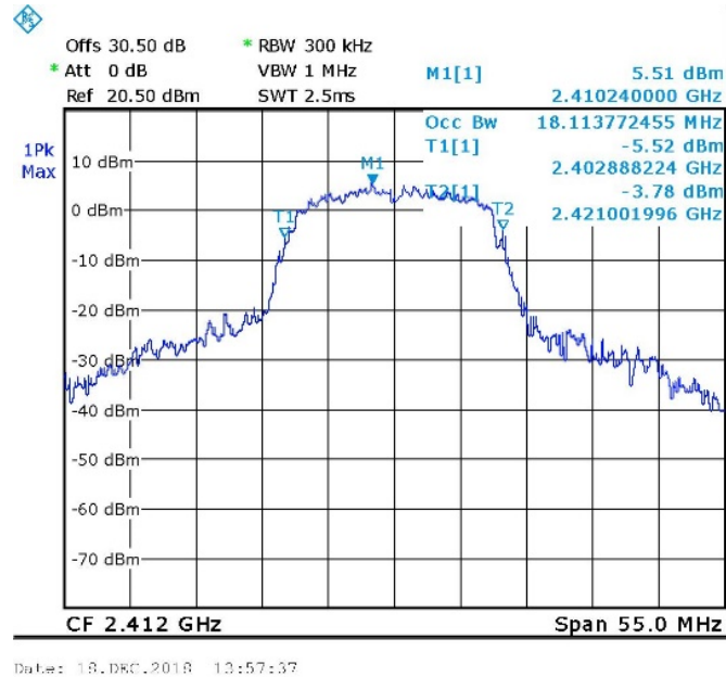
Figure 105. 2412.0 MHz, Wi-fi/g(54Mbit/s)
