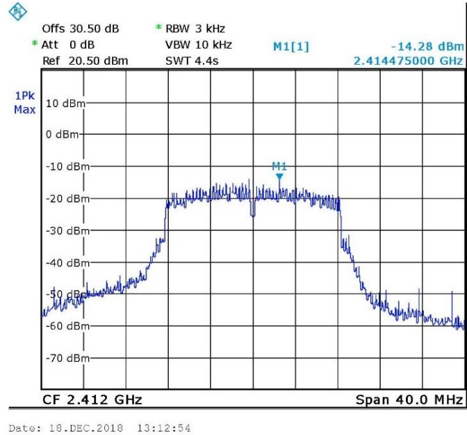
Figure 88. 2412.0 MHz, Wi-fi/g(54Mbit/s)
