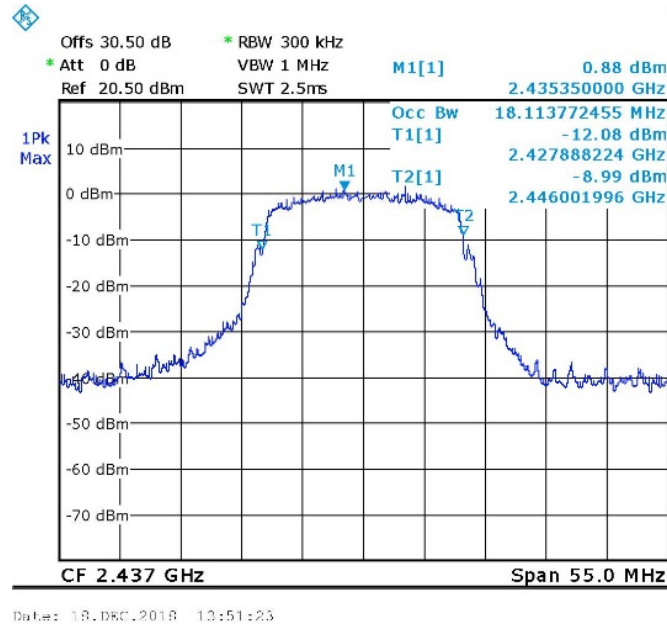
Figure 109. 2437.0 MHz, Wi-fi/n(6.5Mbit/s)
