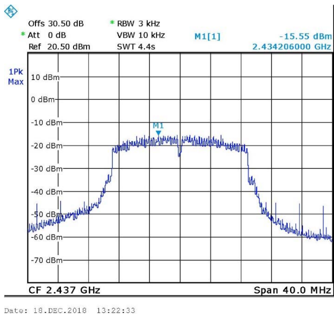
Figure 92. 2437.0 MHz, Wi-fi/n(6.5Mbit/s)
