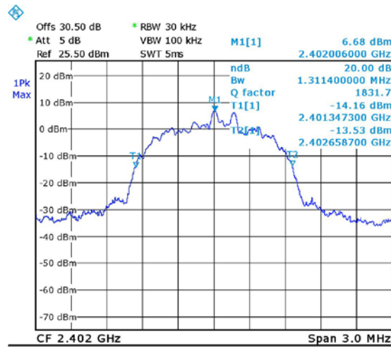
Figure 24. 2402MHz, EDR
