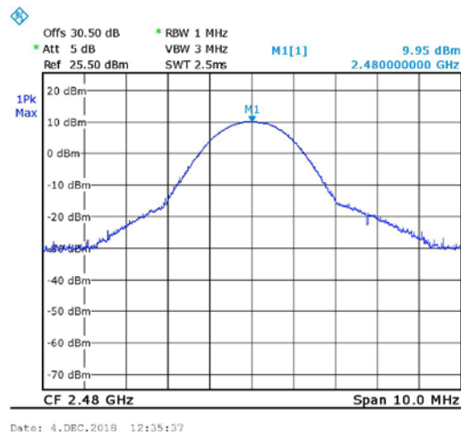
Figure 56. 2480MHz, EDR
