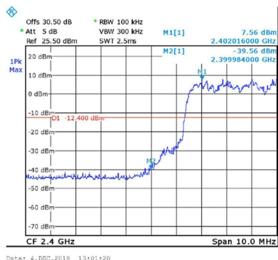
Figure 68 Hopping, Band Edge Low, EDR
