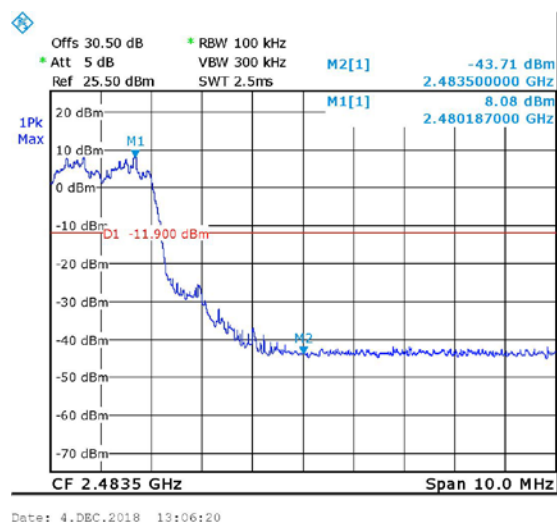
Figure 69 Hopping, Band Edge High, EDR
