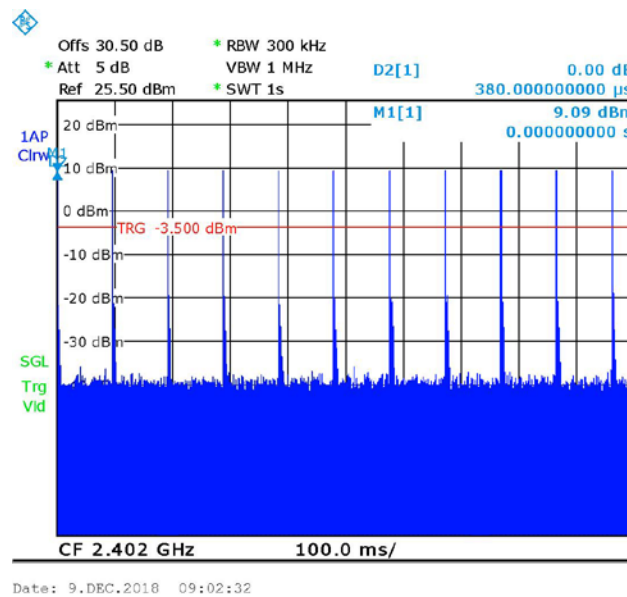
Figure 58 Number of Bursts in 1 sec=11
