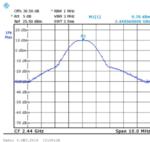
Figure 52. 2440MHz, STD
