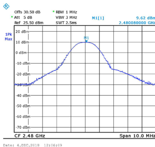
Figure 53. 2480MHz, STD
