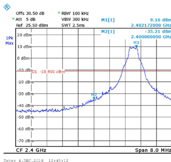
Figure 66 Non-Hopping, Band Edge Low, STD
