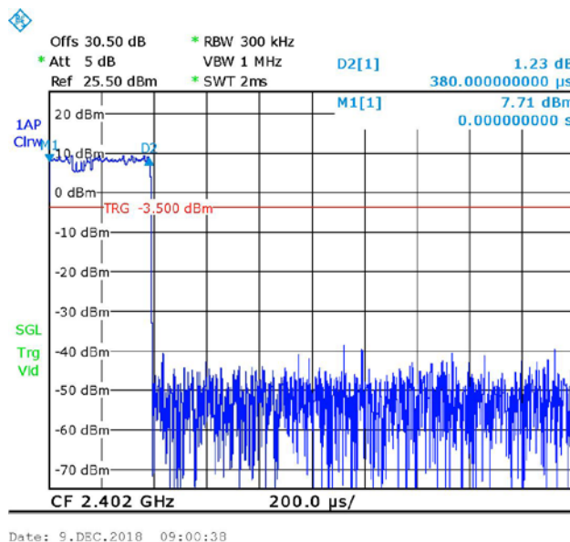
Figure 59 Burst Duration =0.38msec DWELL TIME (31.6*11)*0.38m= 132msec<400msec
