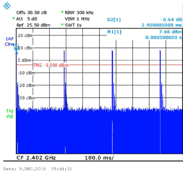
Figure 60 — Number of Bursts in 1 sec=4
