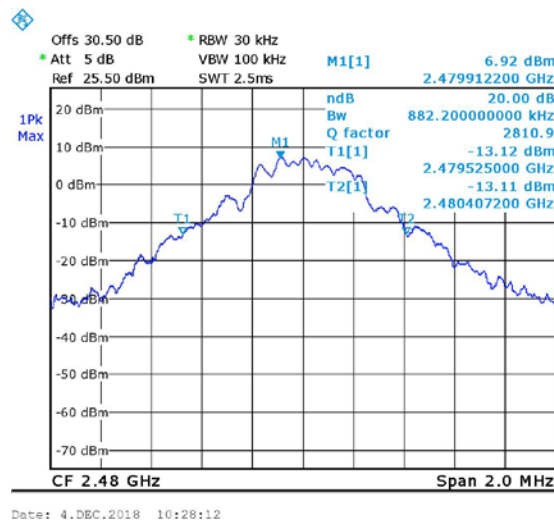
Figure 23. 2480MHz, STD
