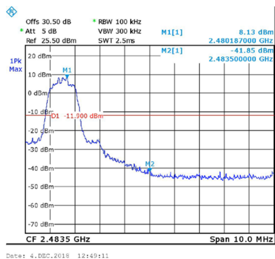
Figure 71 Non-Hopping, Band Edge High, EDR
