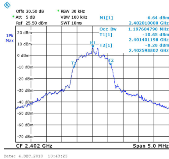
Figure 32. 2402MHz, EDR
