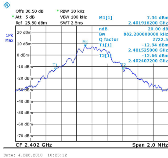
Figure 21. 2402MHz, STD
