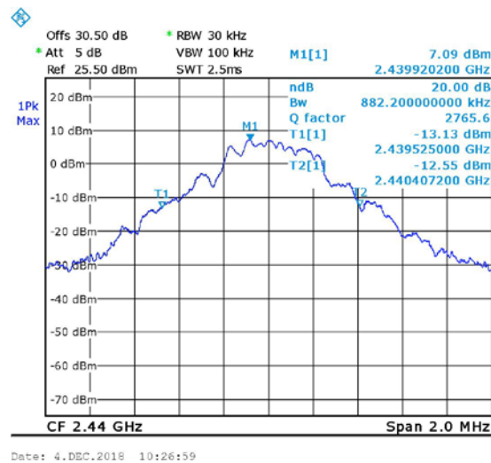
Figure 22. 2440MHz, STD
