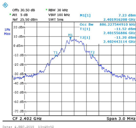
Figure 29. 2402MHz, STD
