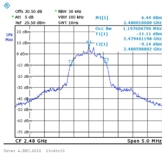
Figure 34. 2480MHz, EDR
