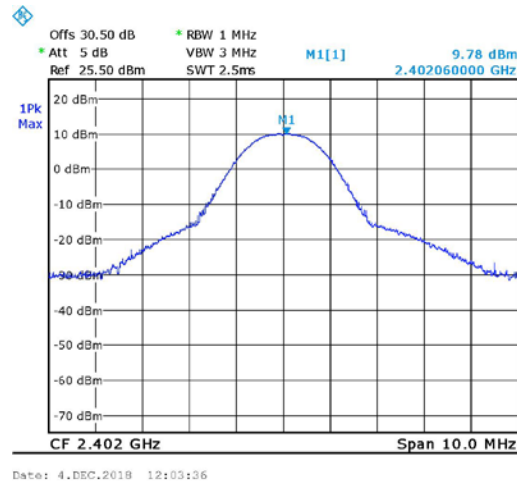
Figure 51. 2402MHz, STD
