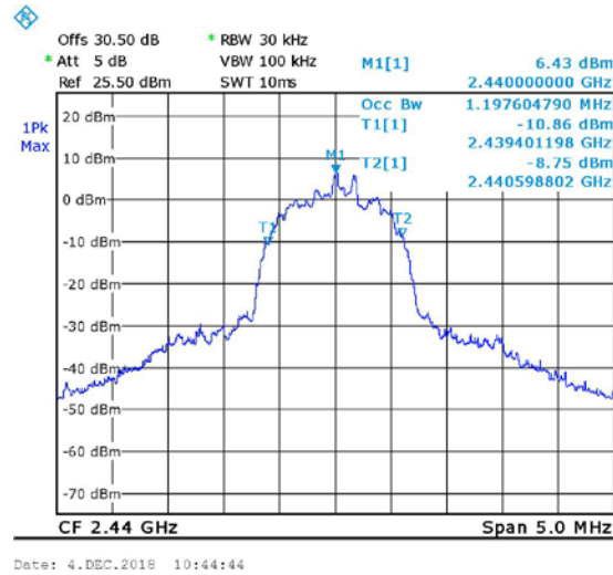
Figure 33. 2440MHz, EDR
