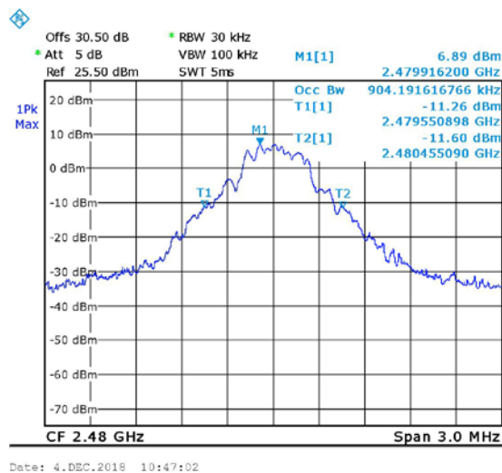
Figure 31. 2480MHz, STD
