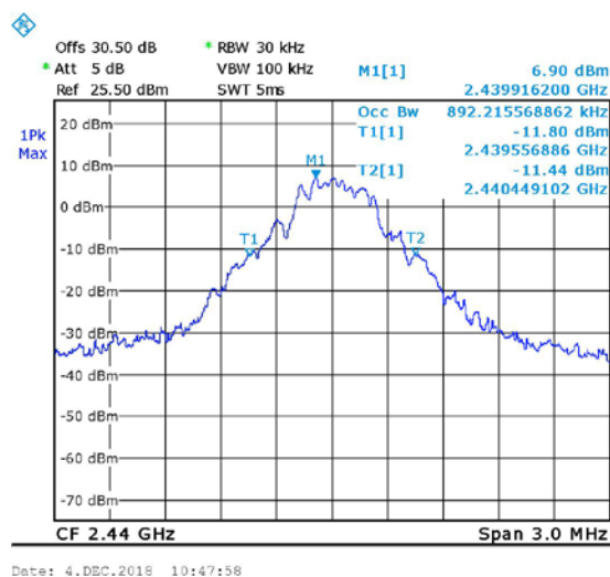
Figure 30. 2440MHz, STD
