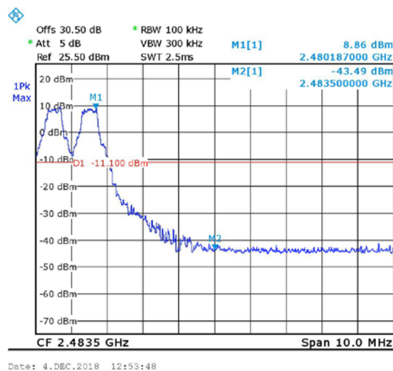
Figure 65 Hopping, Band Edge High, STD
