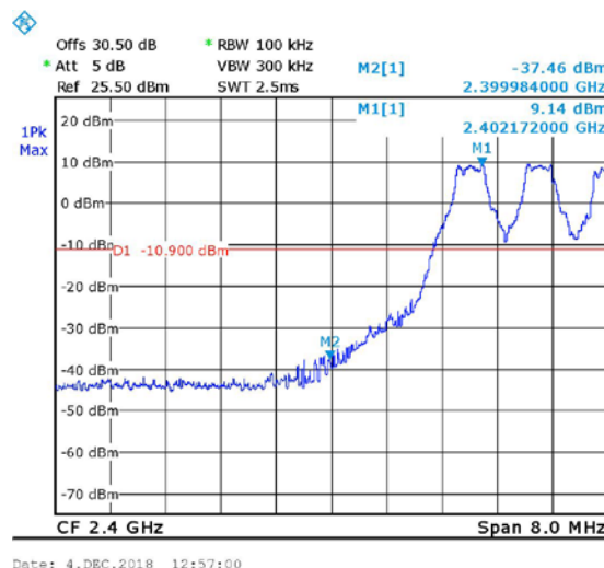
Figure 64 Hopping, Band Edge Low, STD
