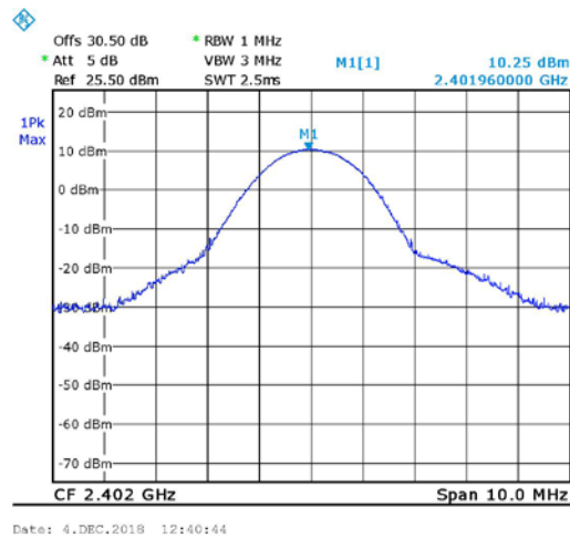
Figure 54. 2402MHz, EDR
