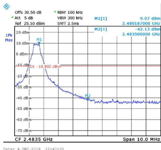
Figure 67 Non-Hopping, Band Edge High, STD
