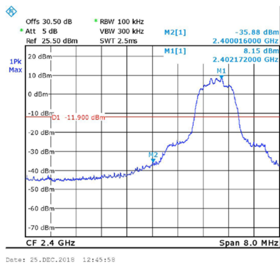
Figure 70 Non-Hopping, Band Edge Low, EDR
