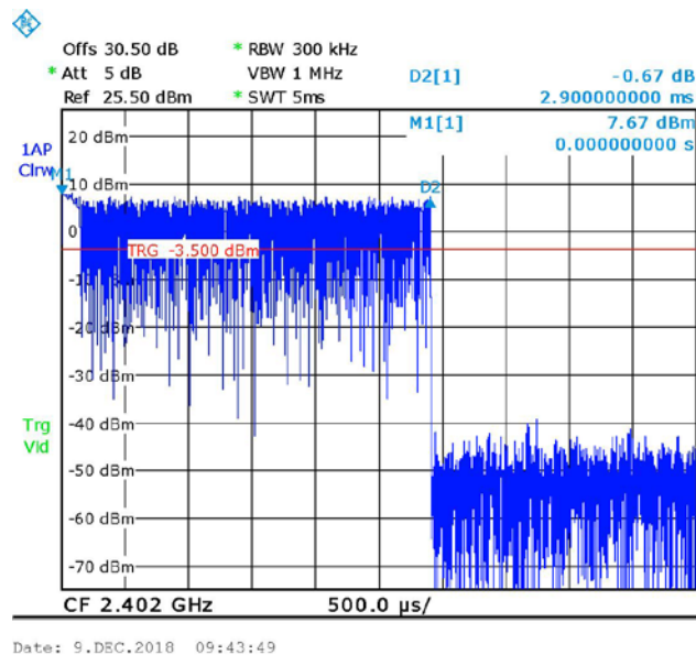
Figure 61 — Burst Duration =2.9msec
