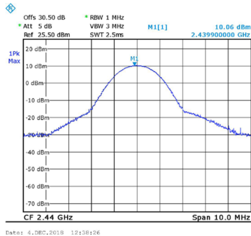
Figure 55. 2440MHz, EDR
