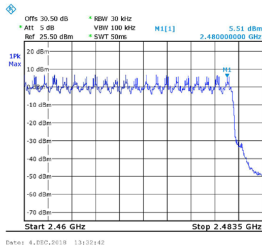
Figure 40. Number of Channels, Band 4, STD
