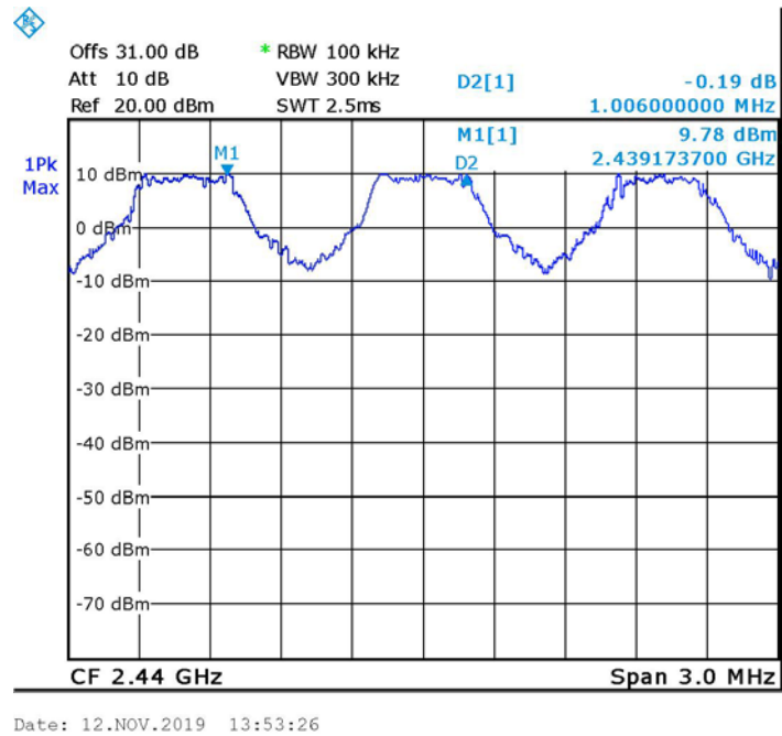
Figure 43. Channel Frequency Separation, STD
