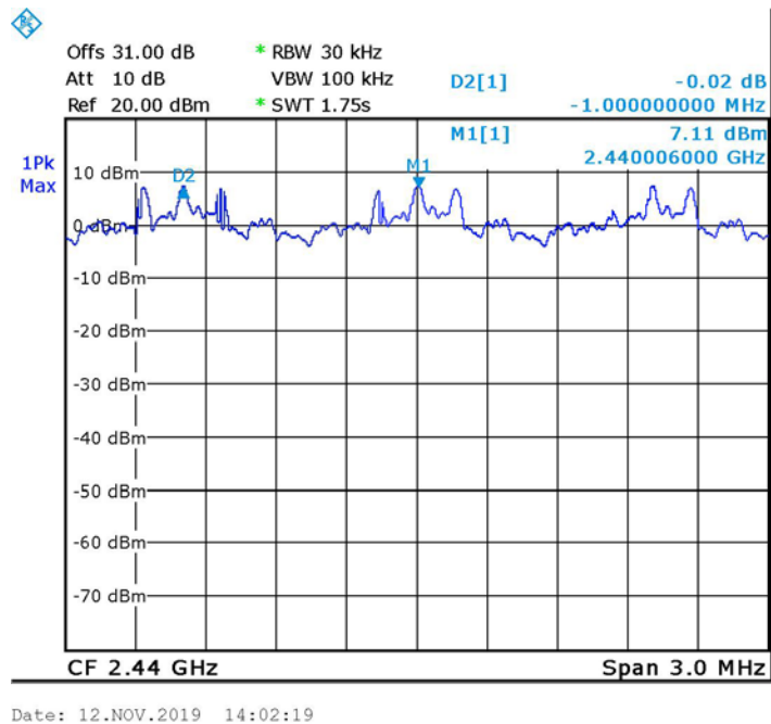
Figure 44. Channel Frequency Separation, EDR
