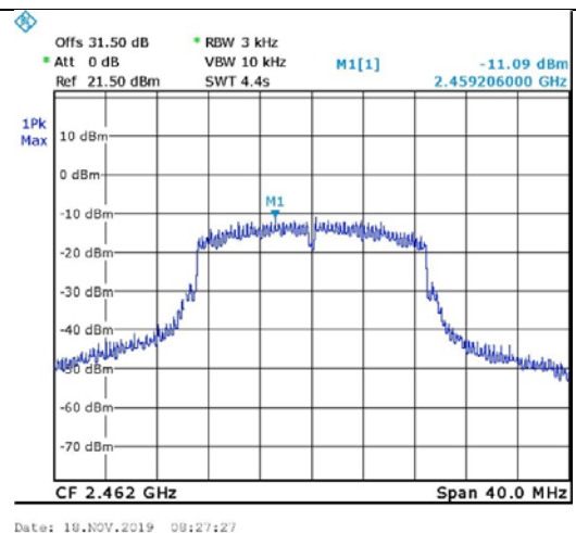
Figure 74. 2462.0 MHz, Wi-fi/n(6.5Mbit/s)
