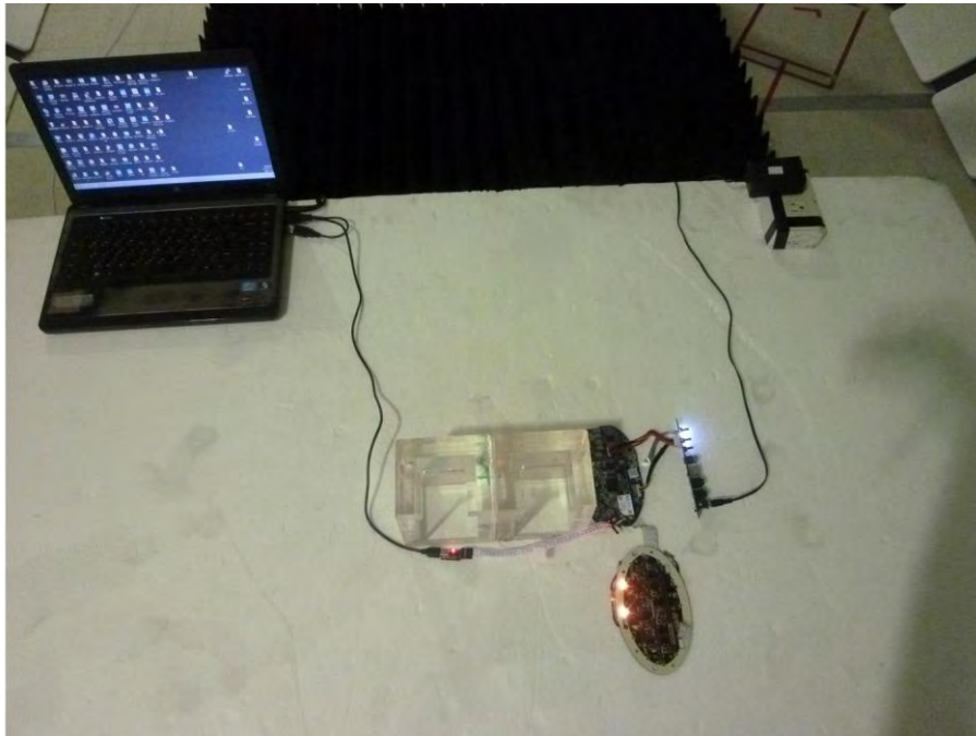
Above 1GHz _ Rear View _ Antenna Model : MSA-3510-25GC4-A25 / MSA-3510-25GC4-A26
