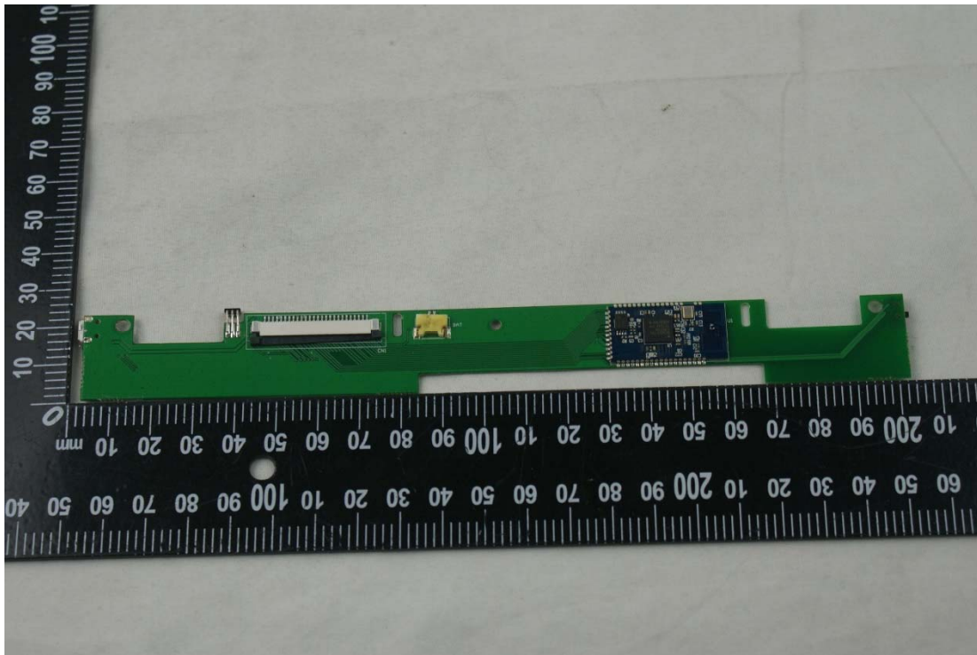
EUT Internal Photo 1
