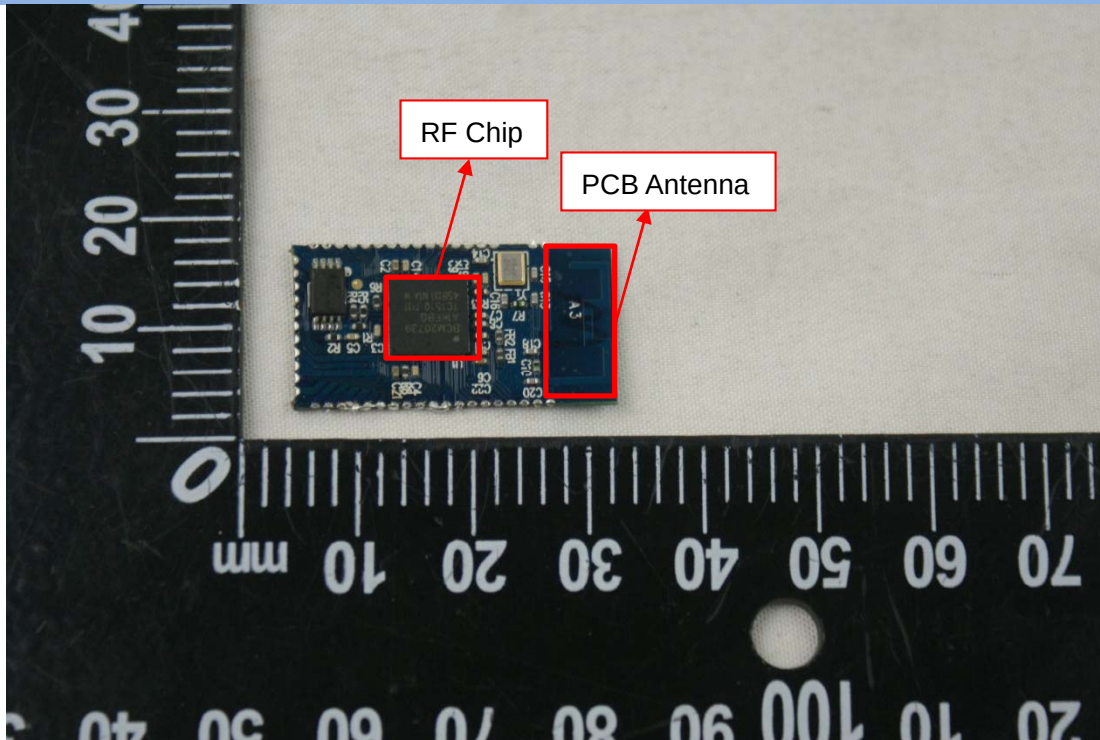
EUT Internal Photo 3
