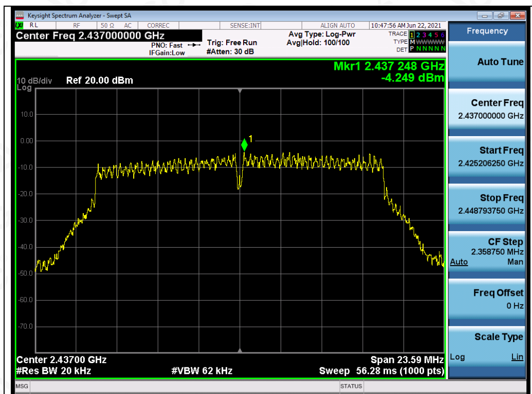
Test_Graph_802.11g_ANT1_2437_6Mbps_PSD
