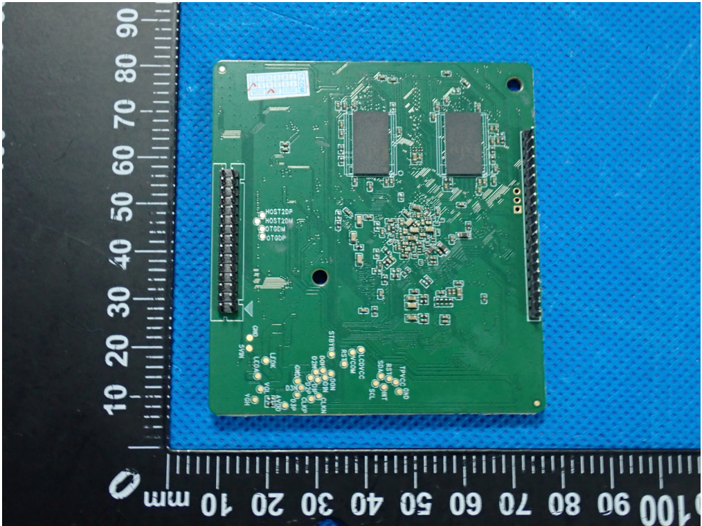
Internal Photo 13
