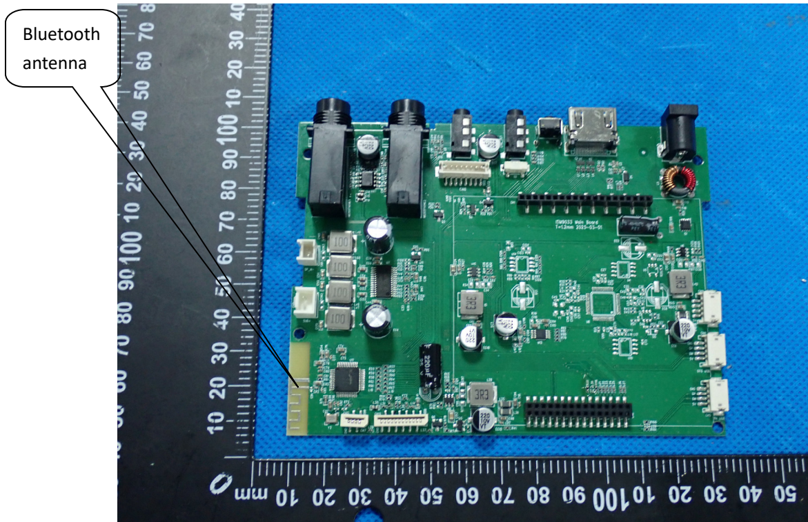
Internal Photo 9
