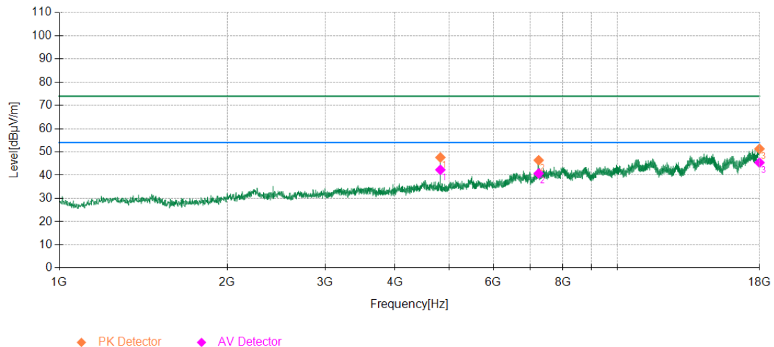
Low Channel - 1-18 GHz - Horizontal
