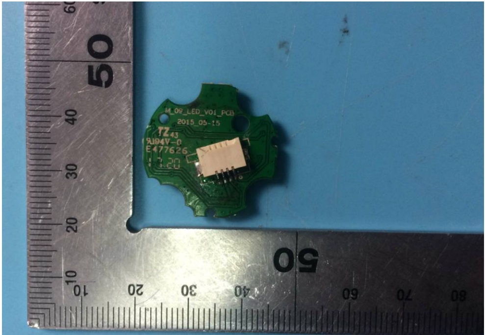
INTERNAL PHOTO OF SAMPLE – 3
