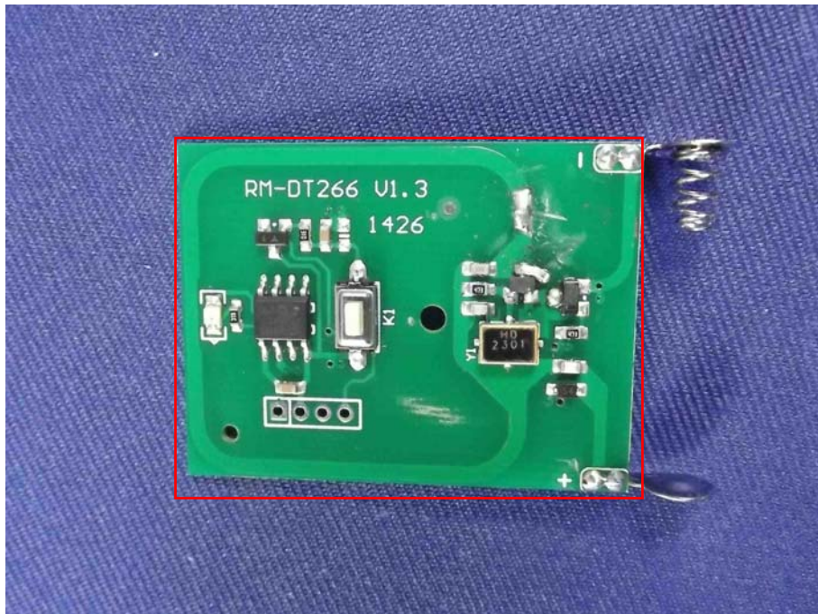
Figure 10 PCB of The EUT-Antenna View
