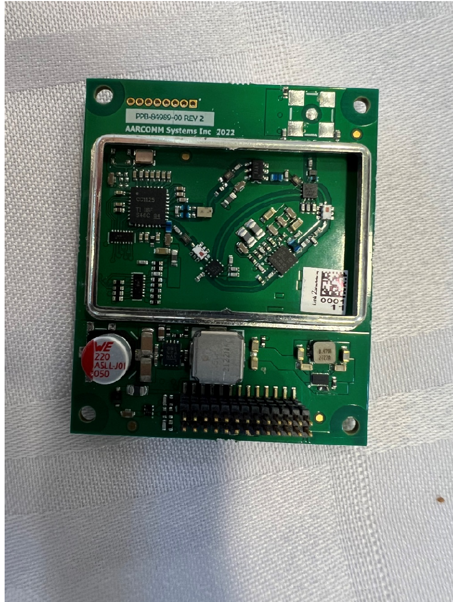
Figure 1 – EUT Internal Photo
