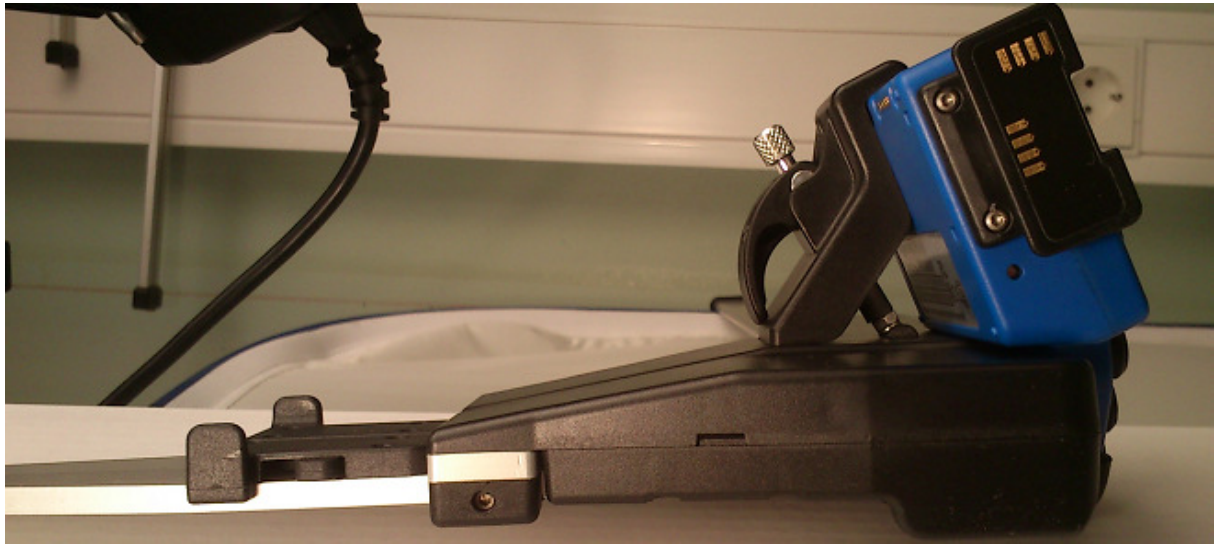
Picture 3. Digitech Professional II , view of left side
