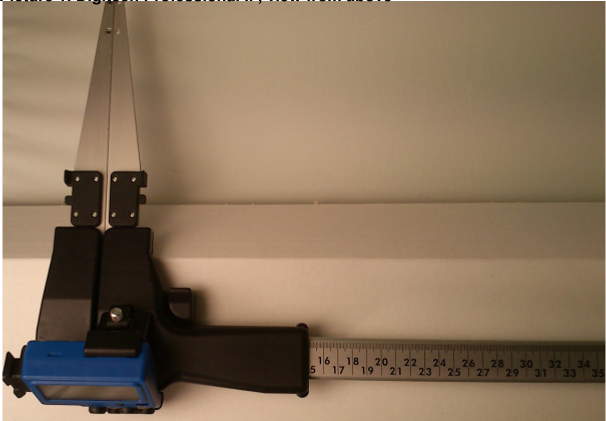
Picture 1. Digitech Professional II , view from above
