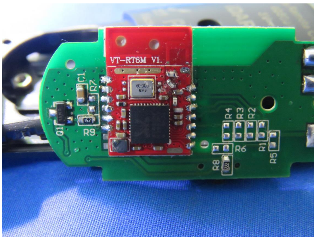
Module (Chip) and Antenna
