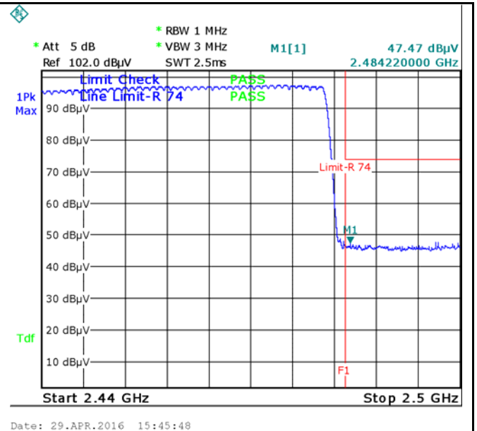
GFSK-Hopping Right Side-PK
