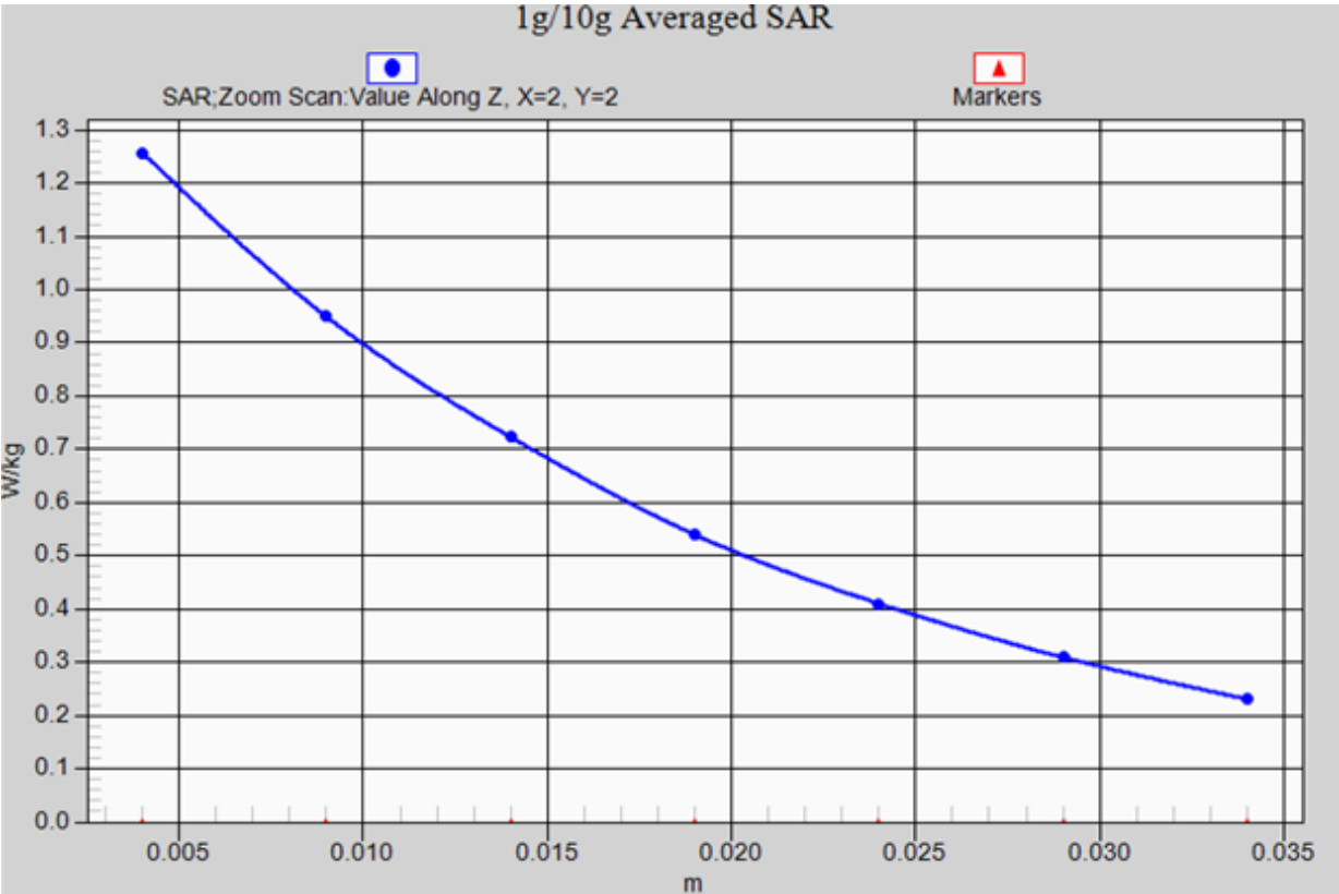
GPRS 850/Back side High- axis scan
