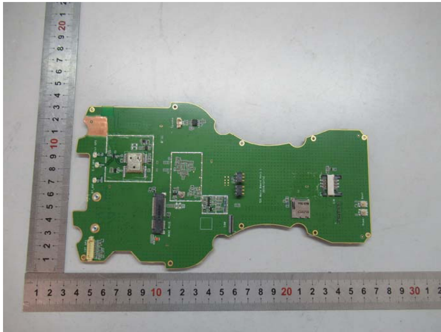
EUT –PCB-3 Bottom (Shielding off) View-3
