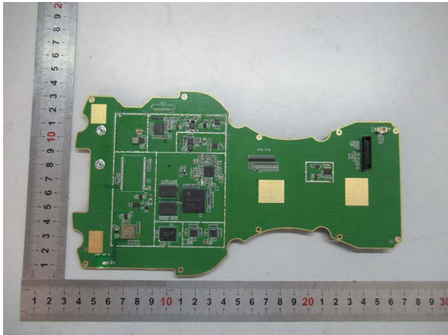
EUT – PCB-3 Top (Shielding off) View
