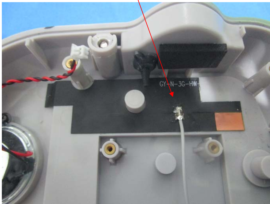
EUT – 2G/3G Antenna View
