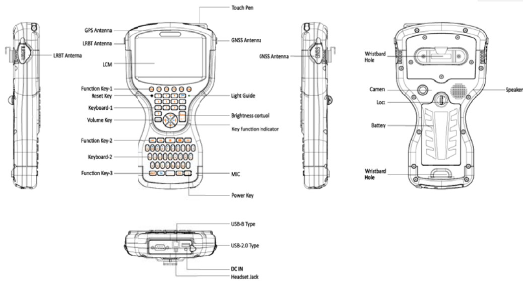
Figure 1-1: General Diagram
