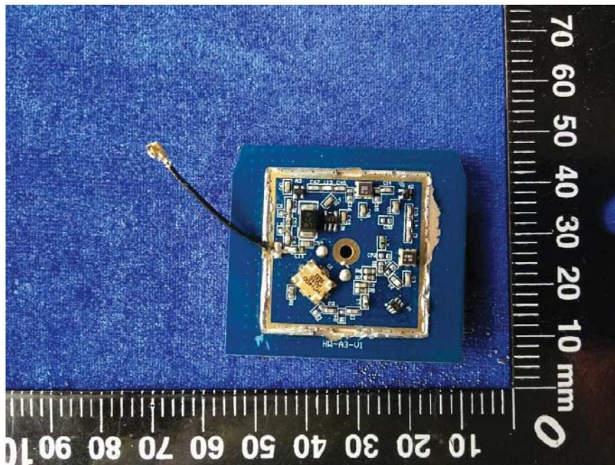
EUT – GPS Module Shielding off View
