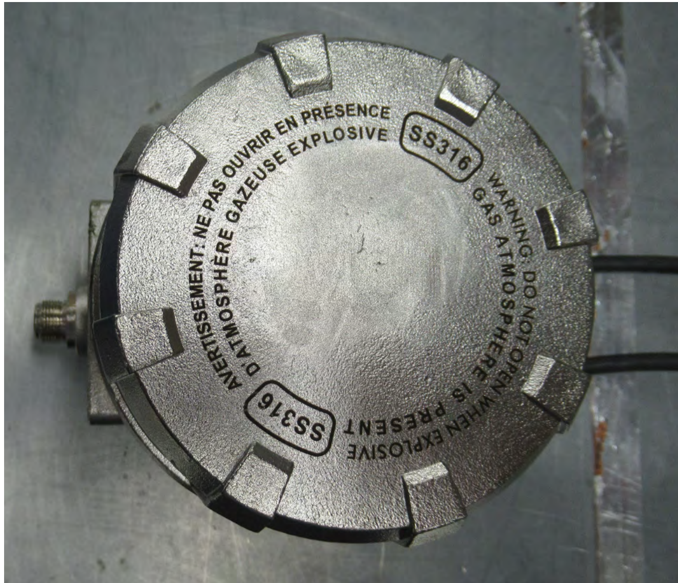
000697 - Bottom View
