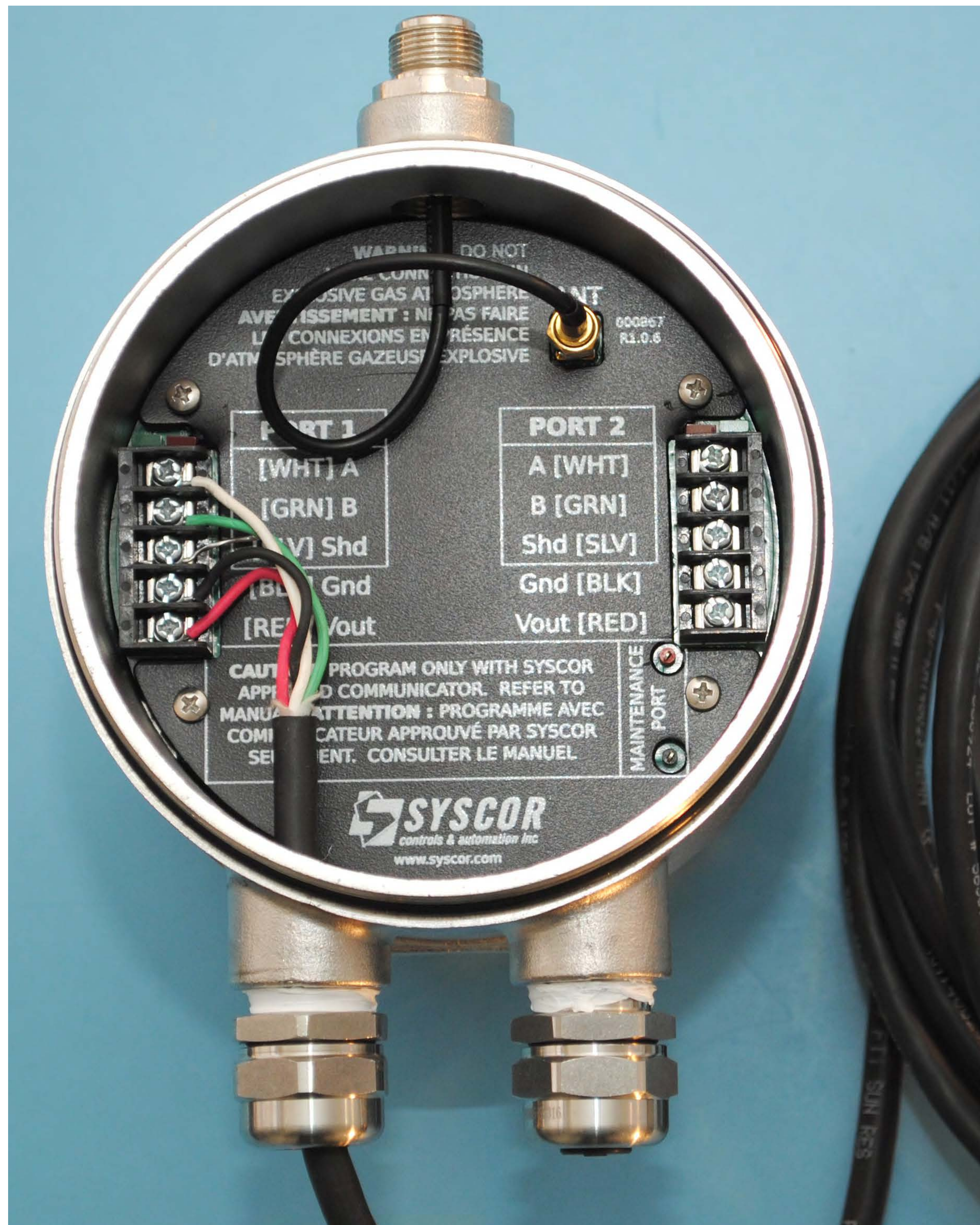
000697 - Bottom View - Label Cover
