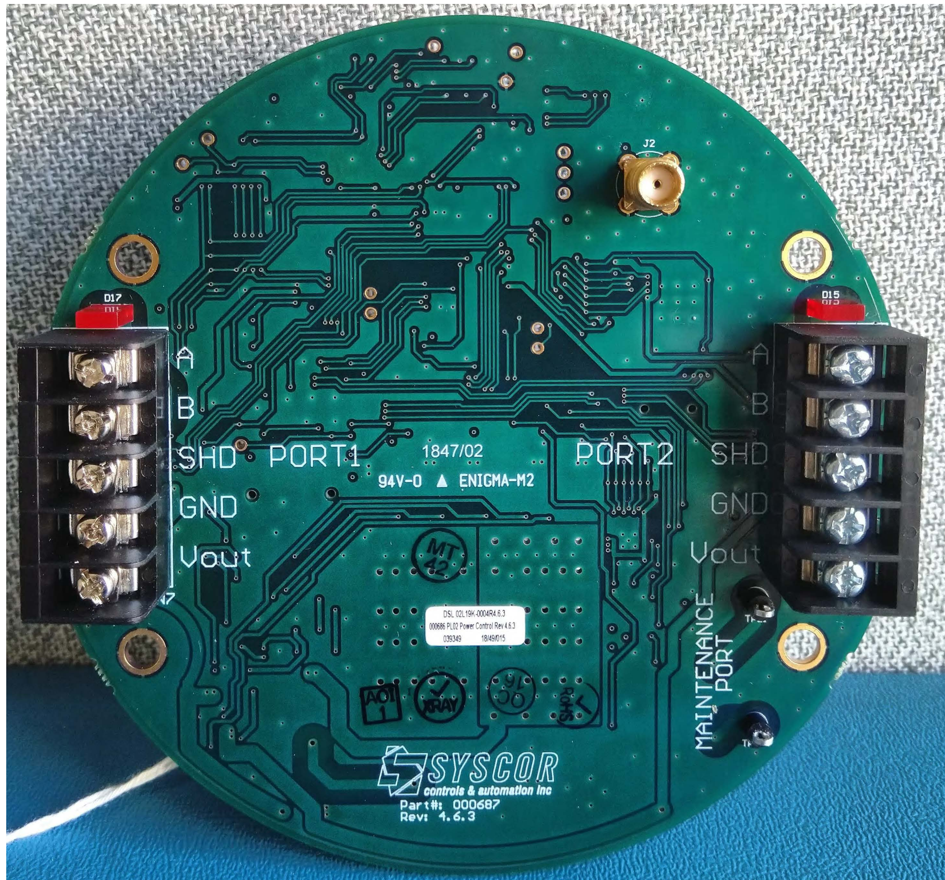
000697 - Bottom View
