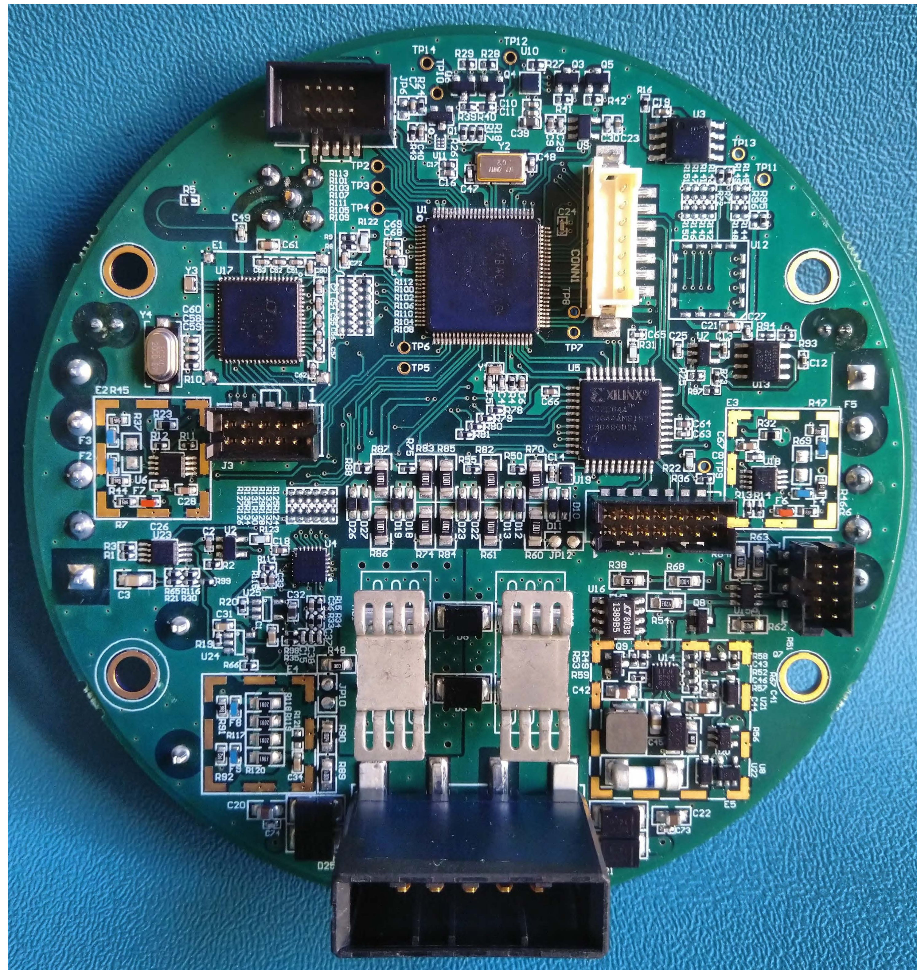
000697 - Top View - shields removed
