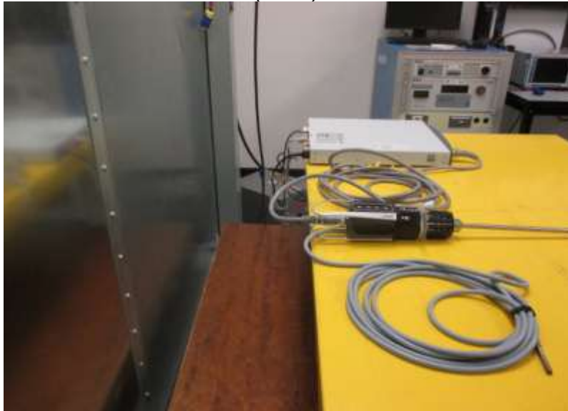
LINE CONDUCTED EMISSION (BACK)
