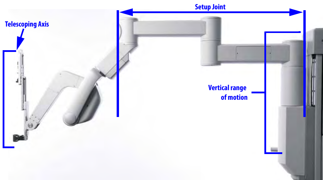
Figure 2.11 setup joint
