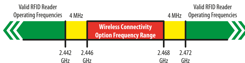
Figure 6 Valid RFID Reader Operating Frequencies
