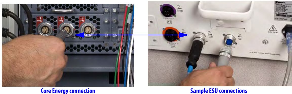
Figure D.11 Example of ESU connection to Core
