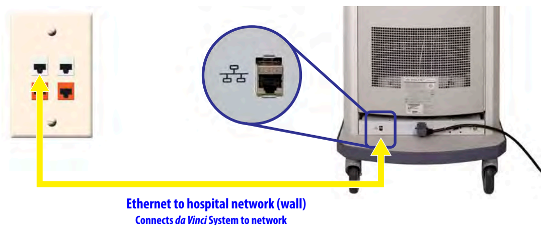
Figure 4 Network Cable Connections (da Vinci Si)
