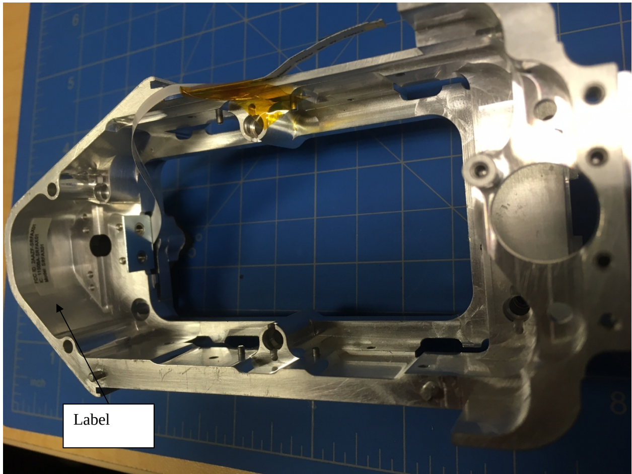
Assembly with flex cable (alternate view)
