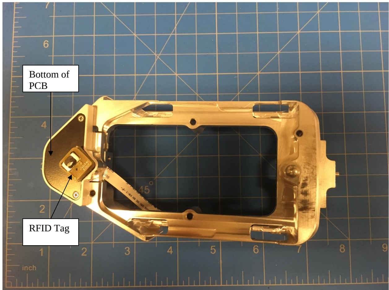
Assembly with RFID tag (top view)
