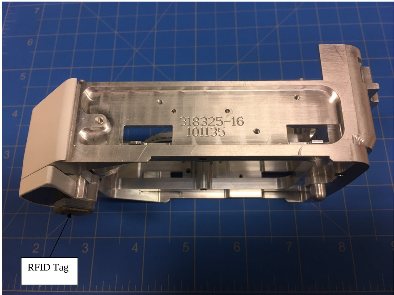
Assembly with RFID tag (side view)
