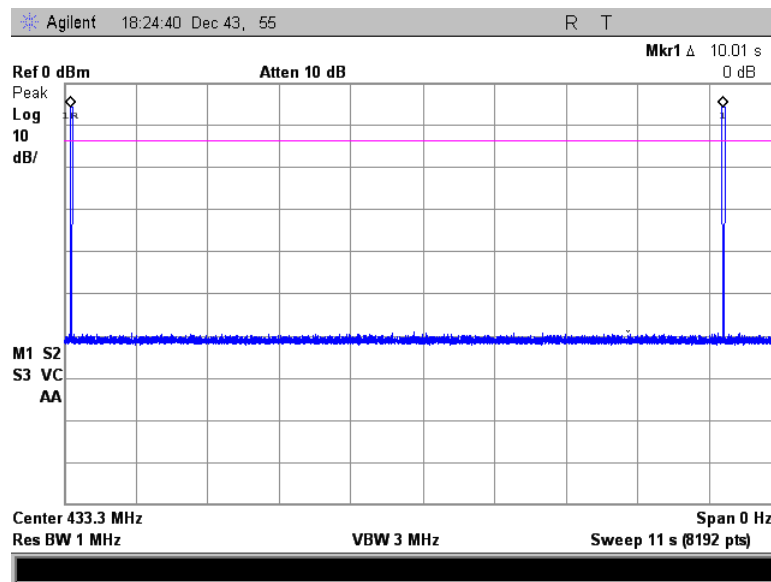
Figure 7.4.2-2: Periodic Operation
