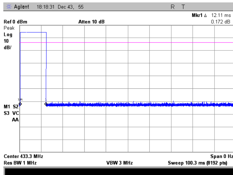
Figure 7.4.2-1: Transmission Duration
