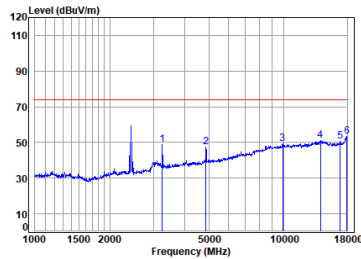
11g_TX_CH_06_Horizontal-Peak
