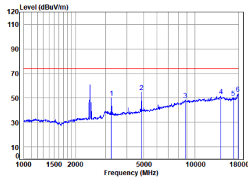
11b_TX_CH_06_Horizontal-Peak
