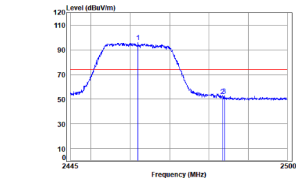
11n_HT(20M)_TX_CH_11_Vertical-Peak
