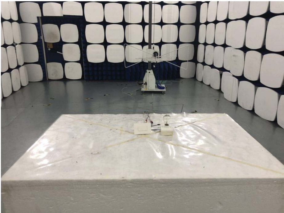
Radiated emission
