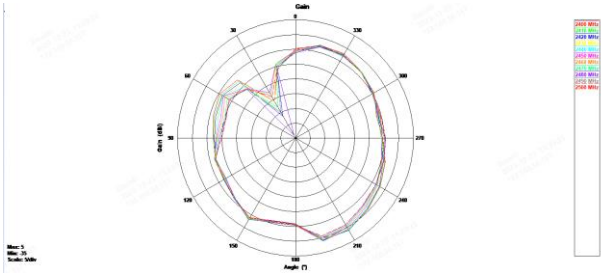
\varphi = 0^\circ (XZ Plane)
