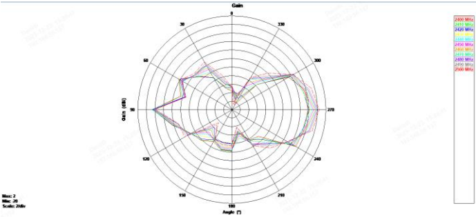
\theta = 90^\circ (XY Plane)
