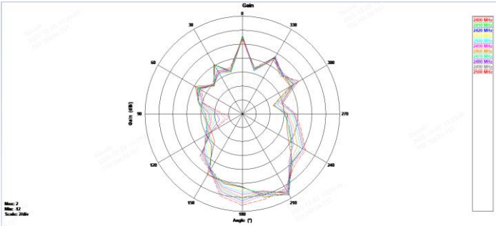
\varphi = 90^\circ (YZ Plane)
