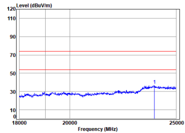
BLE_1M_TX_CH_M_Vertical
