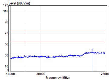
BLE_1M_TX_CH_M_Horizontal
