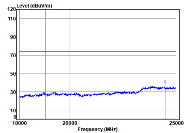
BLE_2M_TX_CH_M_Vertical
