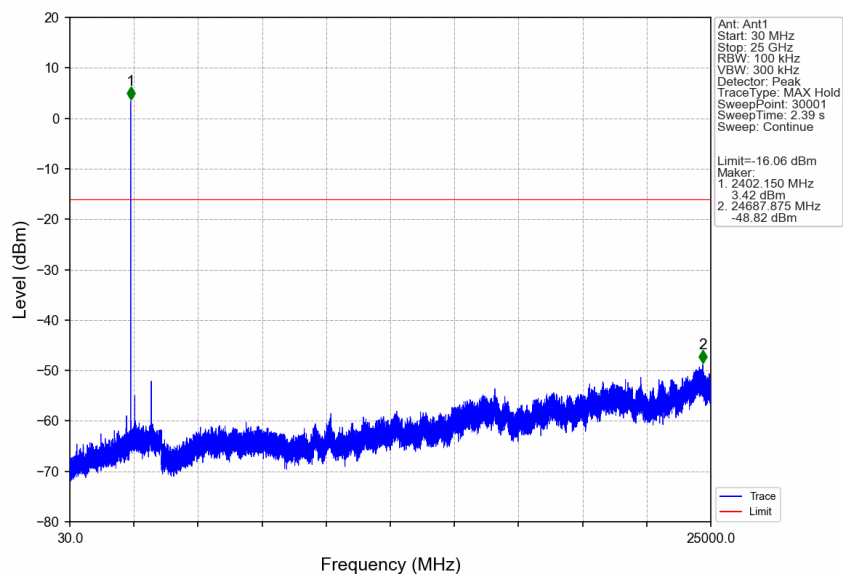
1M_LCH_2402MHz_Ant1_NTNV
