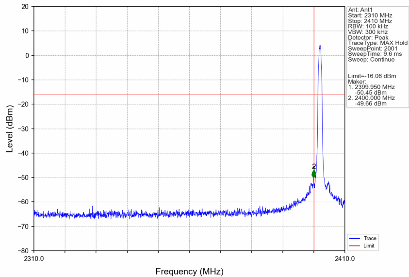
1M_LCH_2402MHz_Ant1_NTNV
