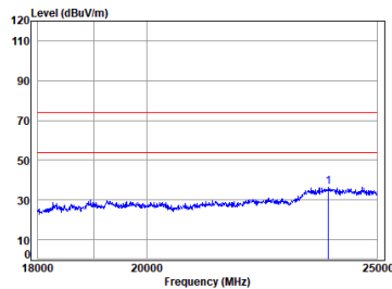
BLE_2M_TX_CH_M_Horizontal
