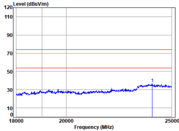
2.4G WIFI_TX_CH_M_Vertical
