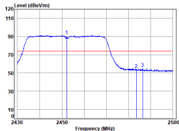
11n_HT(40M)_TX_CH_09_Vertical-Peak
