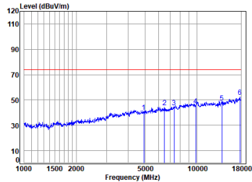
11b_TX_CH_11_Vertical-Peak
