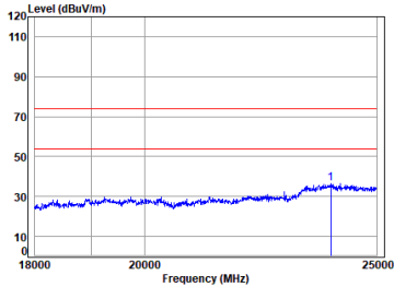
2.4G WIFI_TX_CH_M_Horizontal
