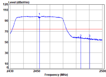
11n_HT(40M)_TX_CH_09_Horizontal-Peak
