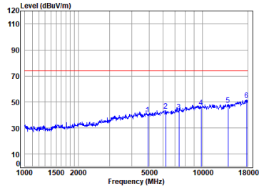
11b_TX_CH_11_Horizontal-Peak
