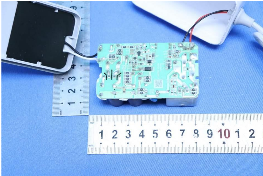
Adapter 2: ZD060CB240200US
