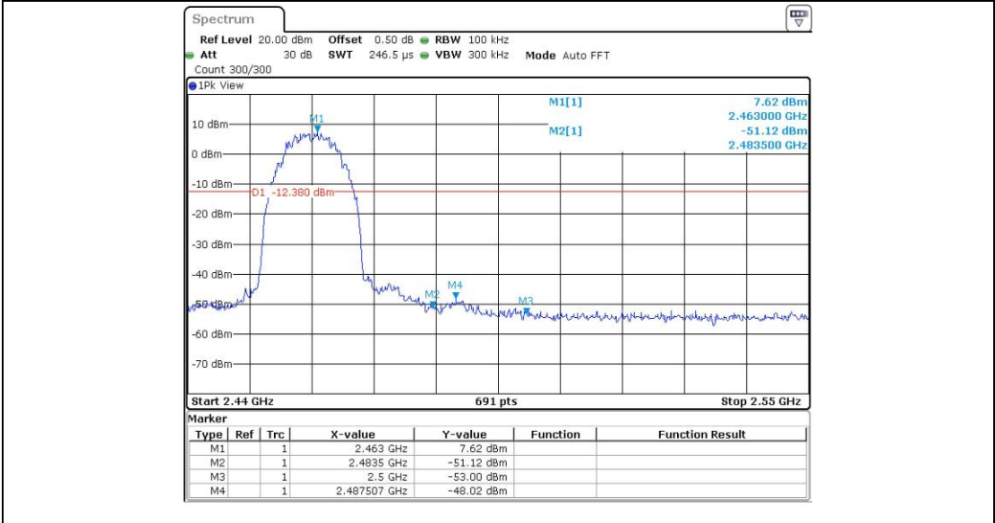
11B_Ant1_High_2462
