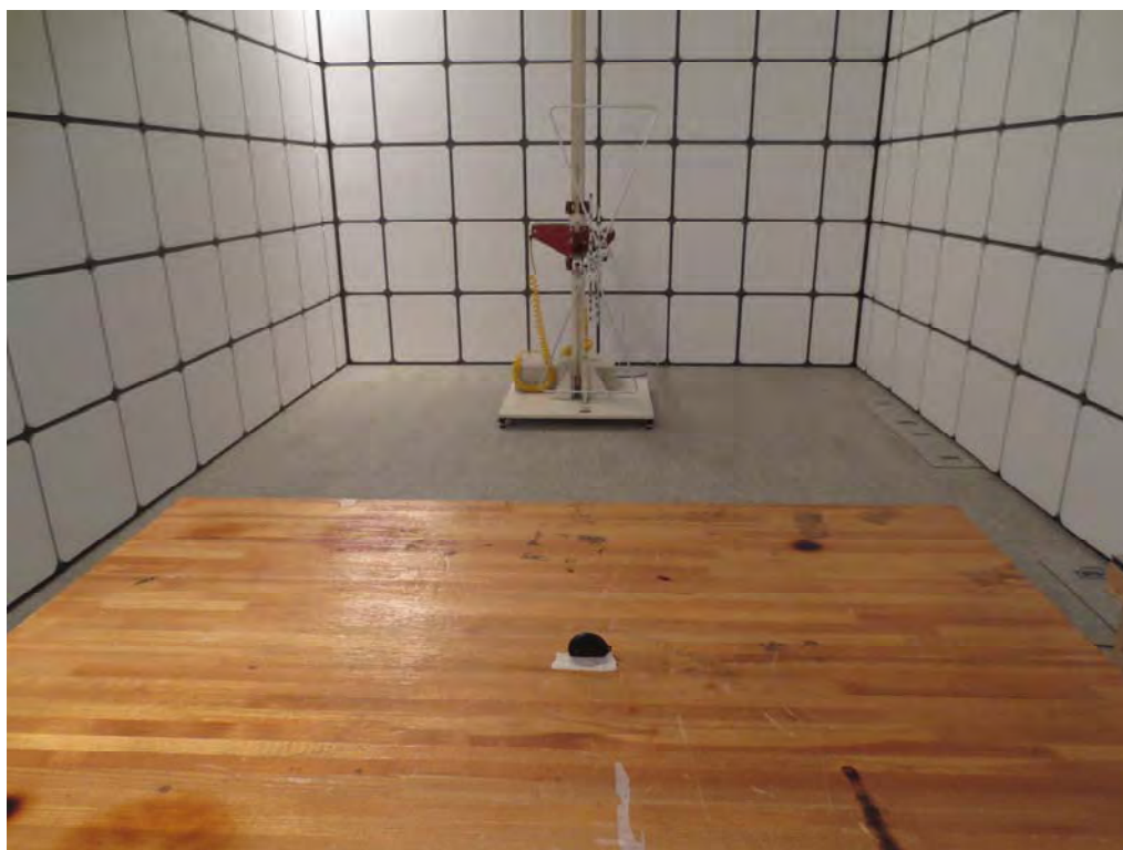
Radiated Emissions Below 1000MHz - Y View
