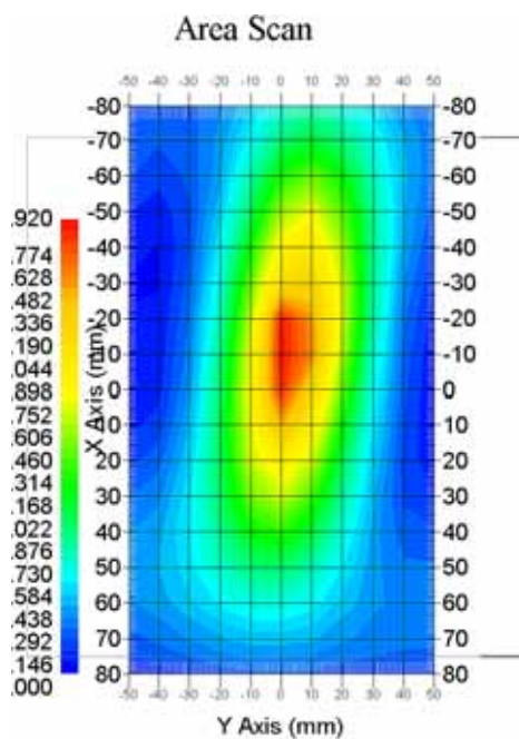
150 MHz System Validation with Head Tissue
