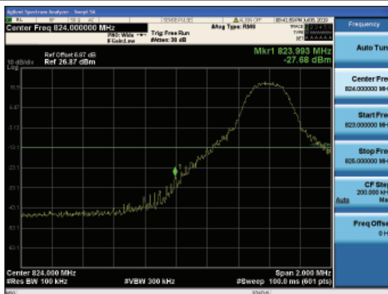
Band26-10MHz-16QAM-26840-1RB#0
