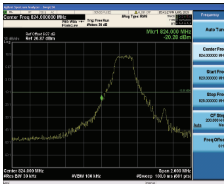
Band26-1.4MHz-16QAM-26797-1RB#0
