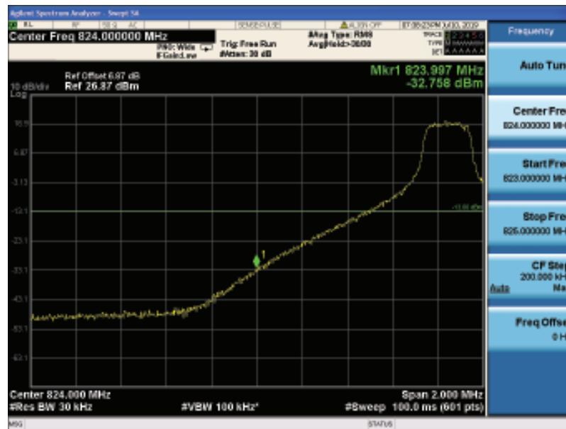
Band26-15MHz-QPSK-26865-1RB#74
