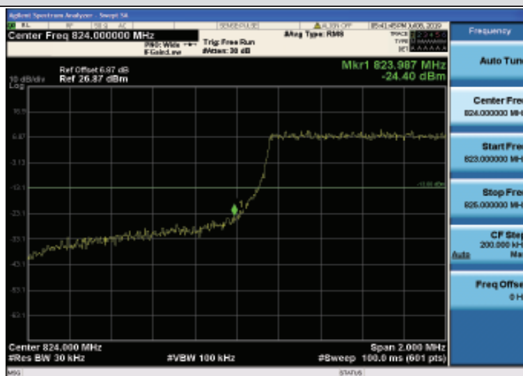
Band26-1.4MHz-16QAM-26797-6RB#0
