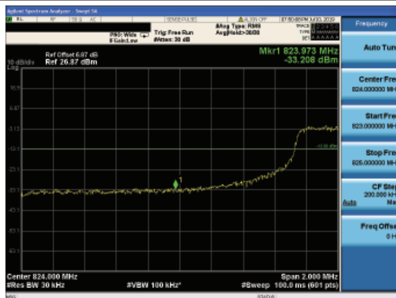
Band26-15MHz-16QAM -26865-75RB#0
