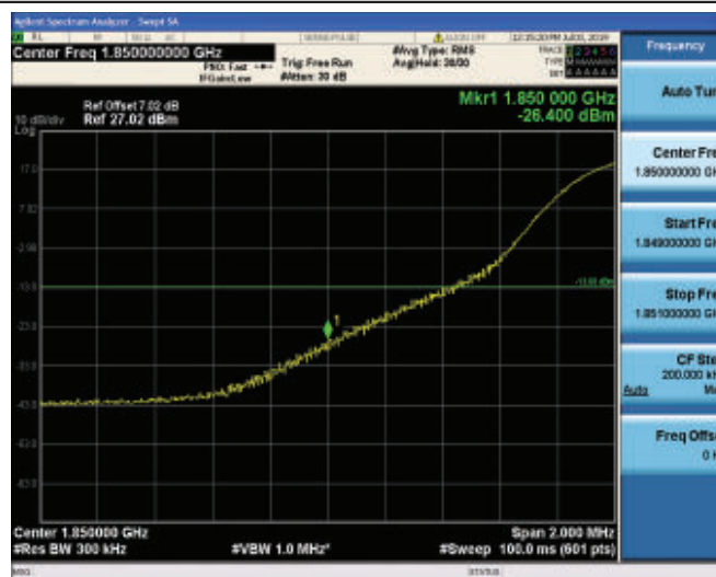
Band25_20MHz_QPSK_26140_1RB#0
