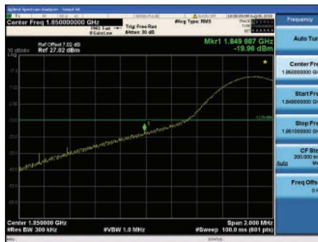
Band25_15MHz_16QAM_26115_1RB#0
