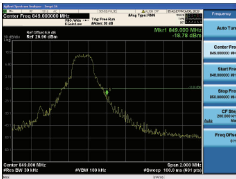
Band26-1.4MHz-16QAM-27033-1RB#5
