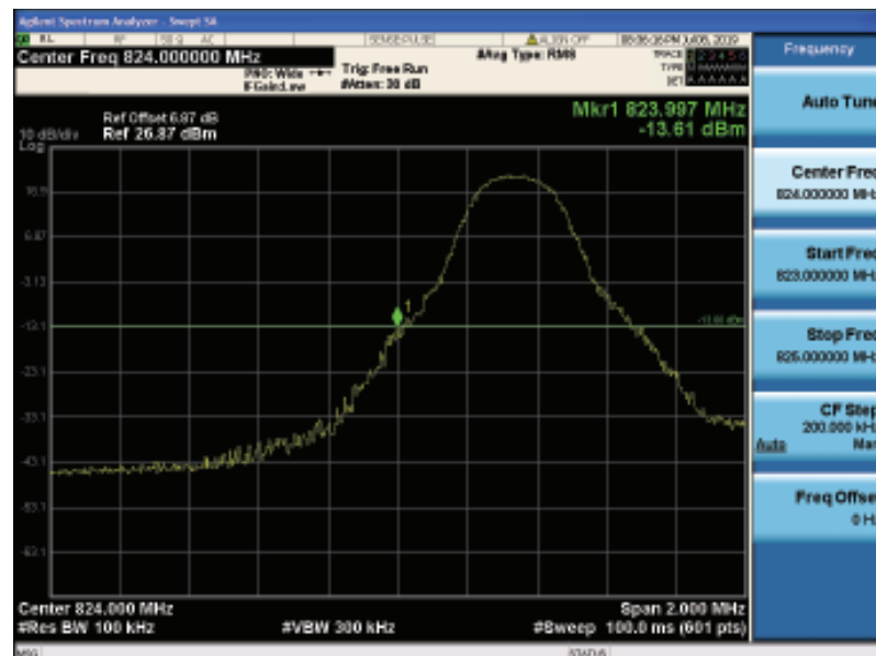
Band26-5MHz-QPSK-26815-1RB#0
