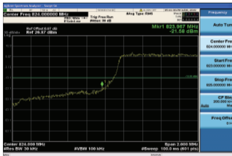
Band26-1.4MHz-QPSK-26797-6RB#0
