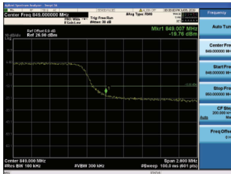
Band26-5MHz-QPSK-27015-25RB#0
