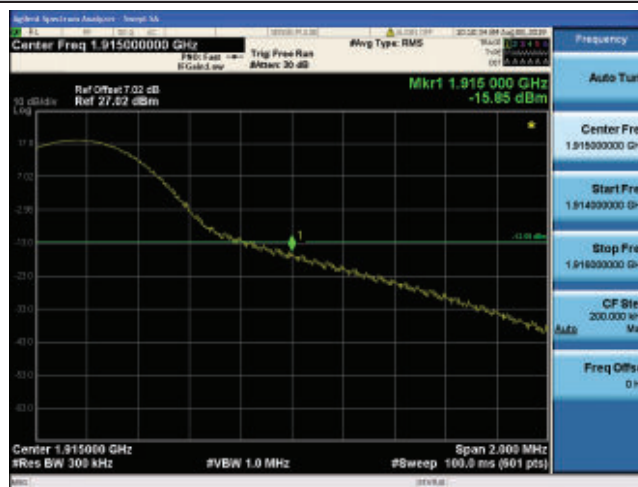
Band25_15MHz_QPSK_26615_1RB#74
