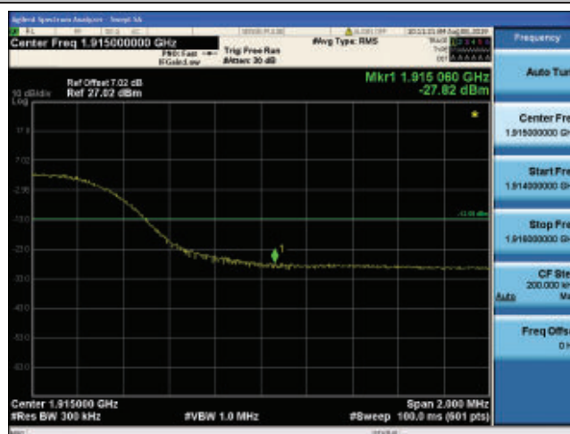
Band25_15MHz_QPSK_26615_75RB#0
