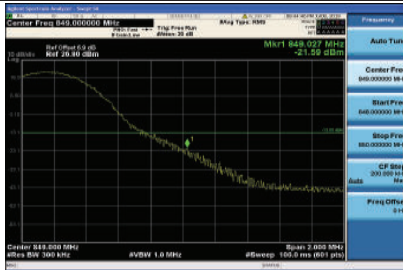
Band26-15MHz-16QAM-26965-1RB#74
