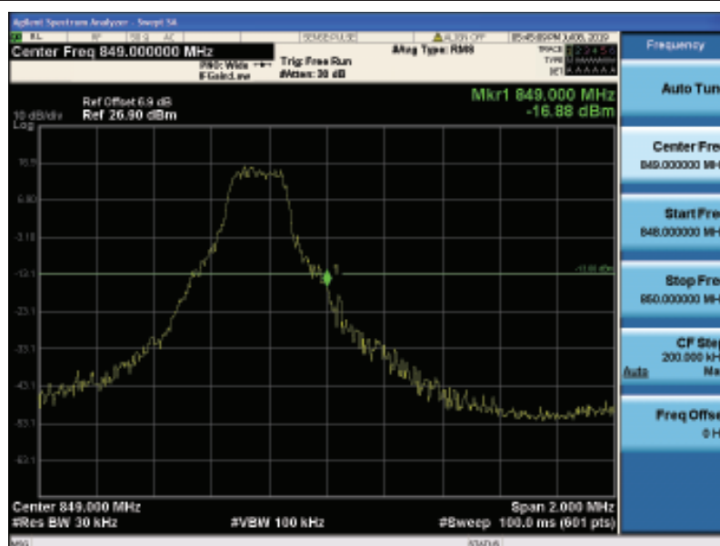
Band26-3MHz-16QAM-27025-1RB#14
