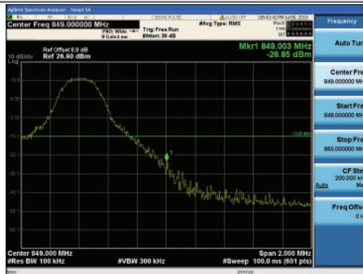
Band26-10MHz-16QAM-26990-1RB#49
