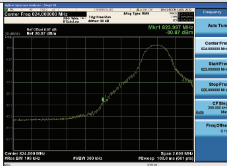
Band26-10MHz-QPSK-26840-1RB#0
