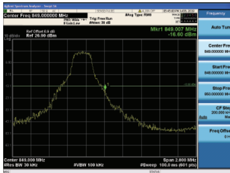
Band26-3MHz-QPSK-27025-1RB#14
