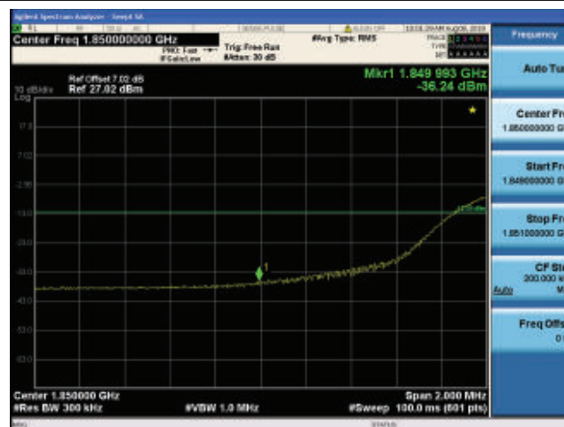
Band25_20MHz_QPSK_26140_100RB#0
