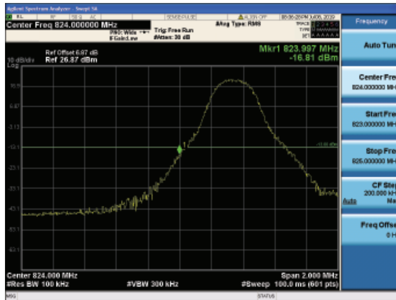
Band26-3MHz-16QAM-26805-1RB#0
