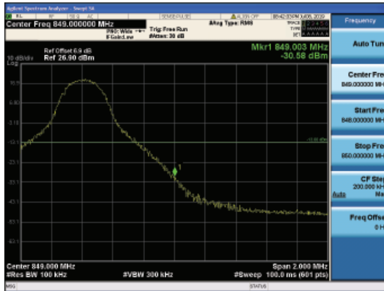
Band26-10MHz-QPSK-26990-1RB#49
