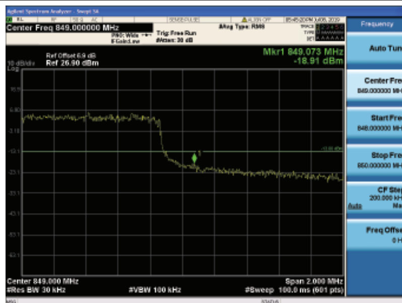
Band26-3MHz-QPSK-27025-15RB#0
