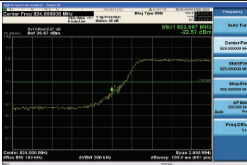
Band26-5MHz-16QAM-26815-25RB#0
