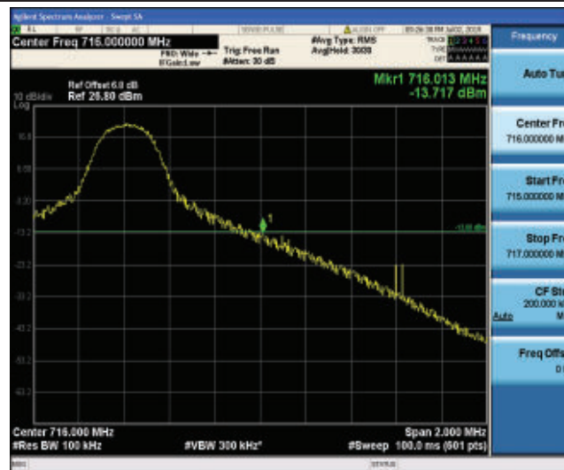
Band12_10MHz_QPSK_23130_1RB#49
