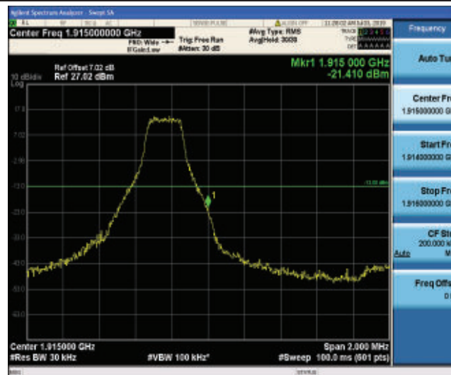
Band25_3MHz_QPSK_26675_1RB#14
