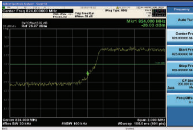
Band26-3MHz-16QAM-26805-15RB#0
