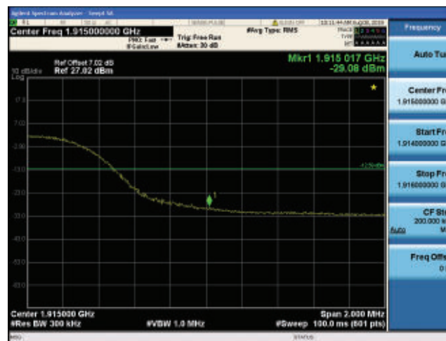
Band25_15MHz_QPSK_26615_75RB#0
