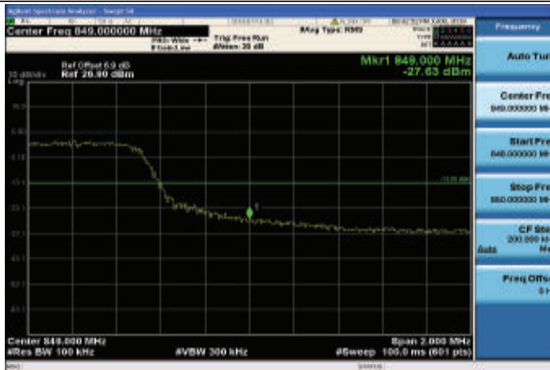
Band26-10MHz-QPSK-26990-50RB#0
