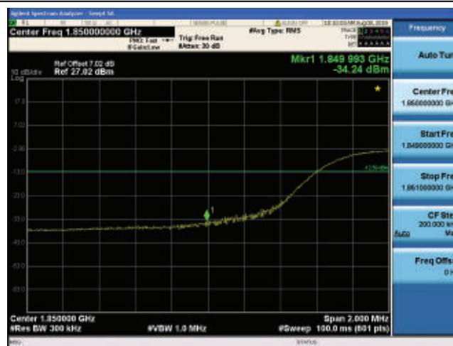
Band25_15MHz_16QAM_26115_75RB#0
