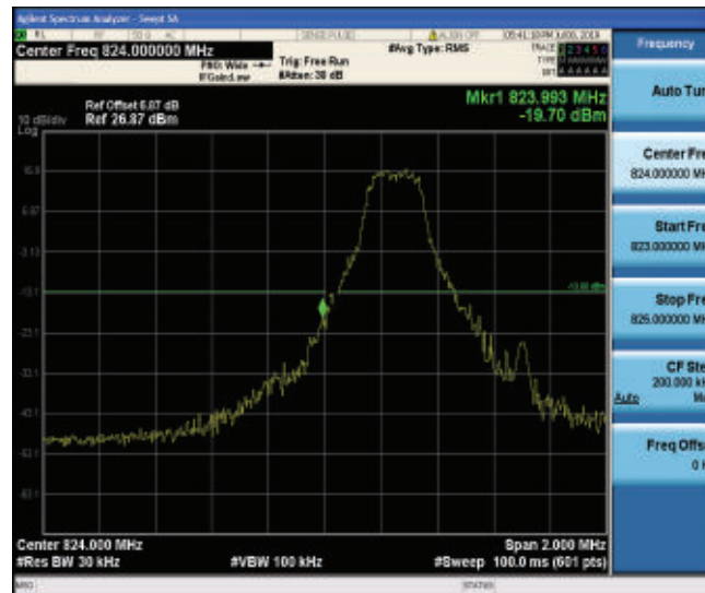
Band26-1.4MHz-QPSK-26797-1RB#0
