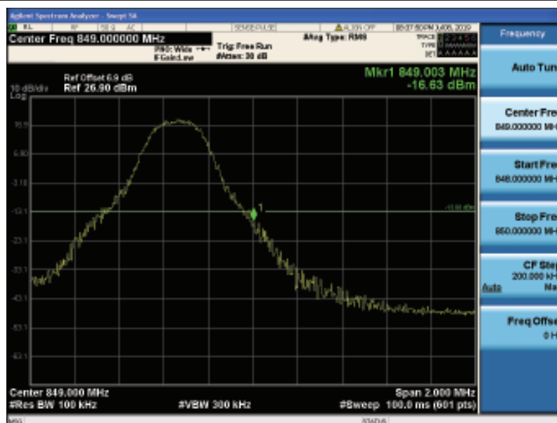
Band26-5MHz-16QAM-27015-1RB#24
