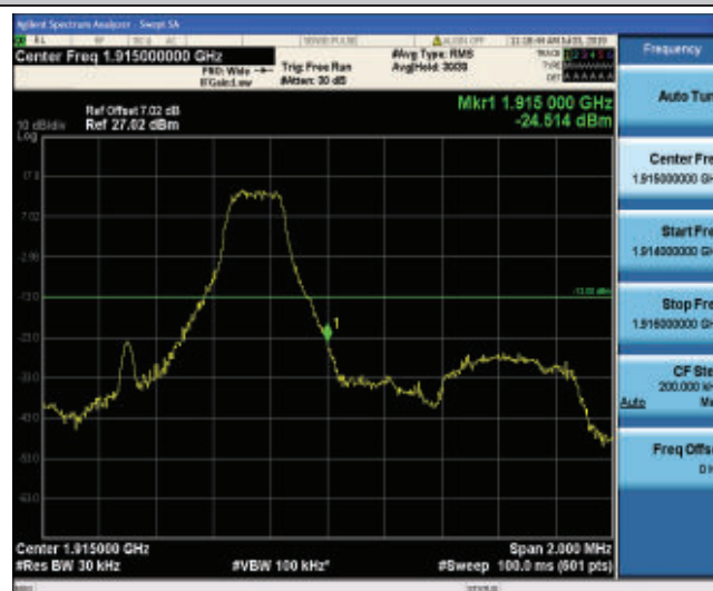
Band25_1.4MHz_QPSK_26683_1RB#5
