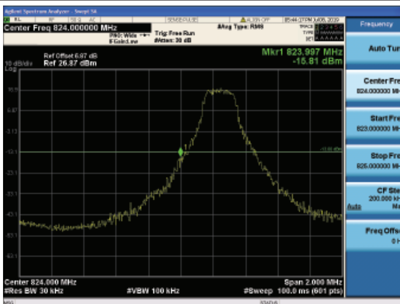
Band26-3MHz-QPSK-26805-1RB#0
