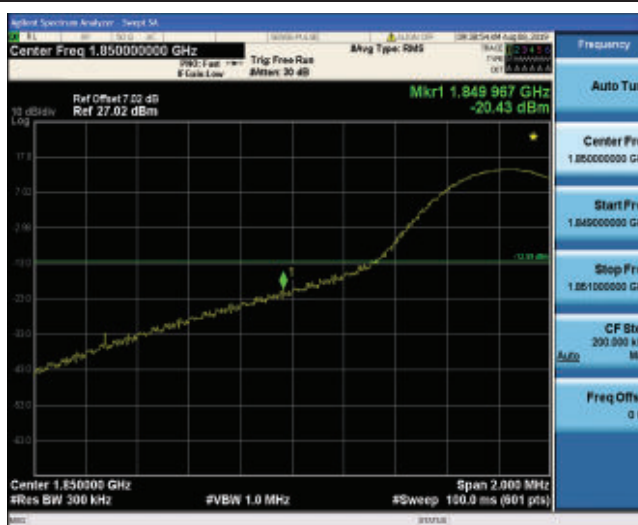
Band25_15MHz_QPSK_26115_1RB#0
