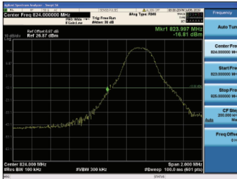
Band26-5MHz-16QAM-26815-1RB#0
