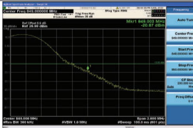
Band26-15MHz-QPSK-26965-1RB#74
