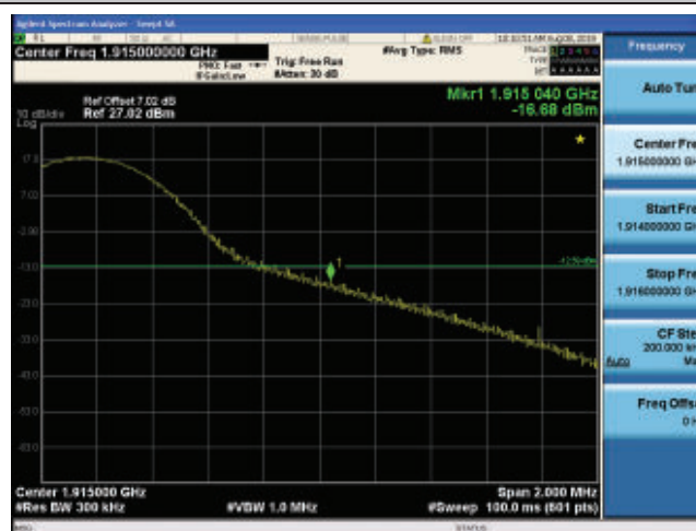
Band25_15MHz_QPSK_26615_1RB#74
