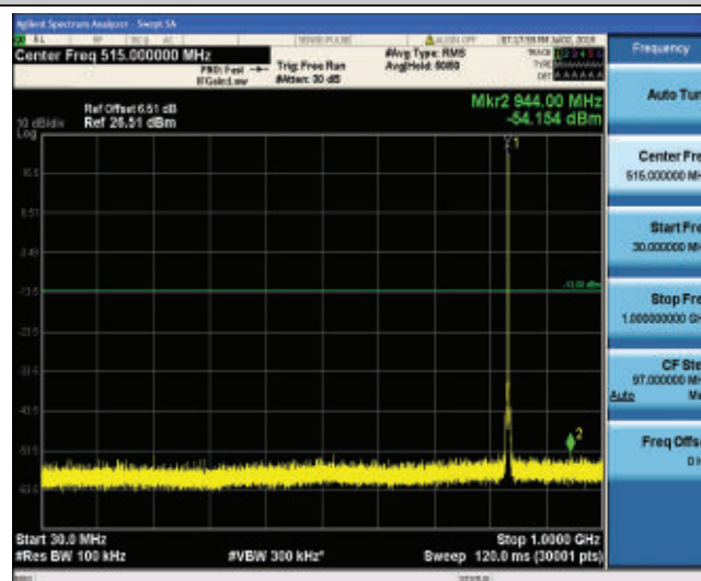
Band5 1.4MHz 16QAM 20525 1RB#0
