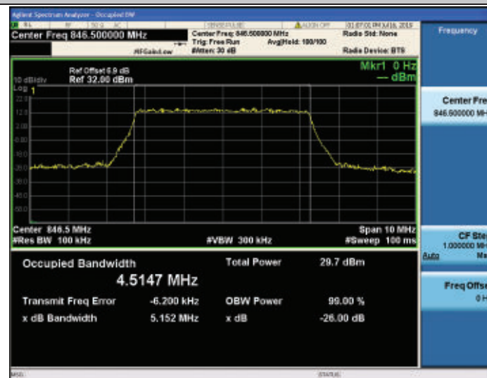
Band26-5MHz-QPSK-27015-25RB#0
