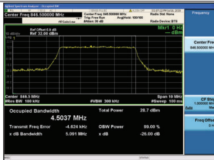
Band26-5MHz-16QAM-27015-25RB#0
