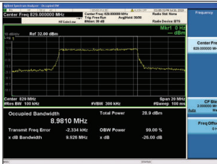
Band26-10MHz-16QAM-26840-50RB#0-8.9810
