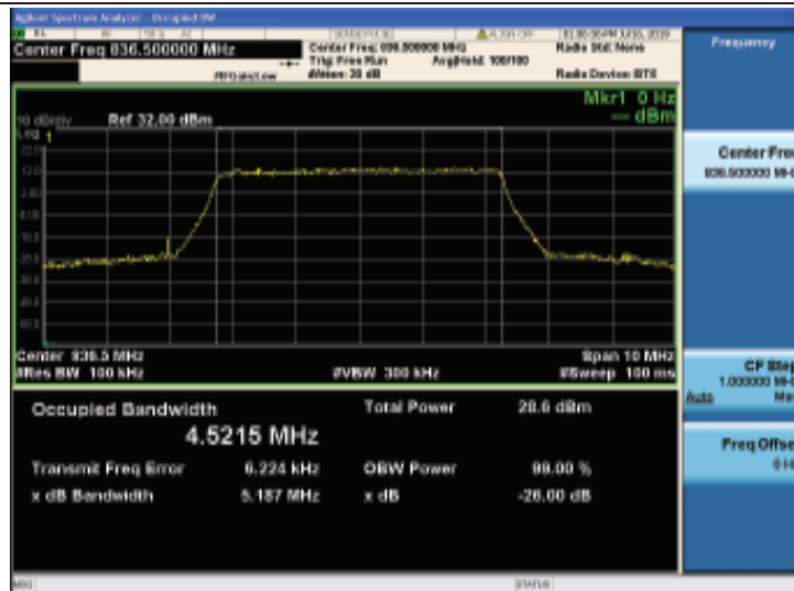
Band26-5MHz-16QAM-26915-25RB#0
