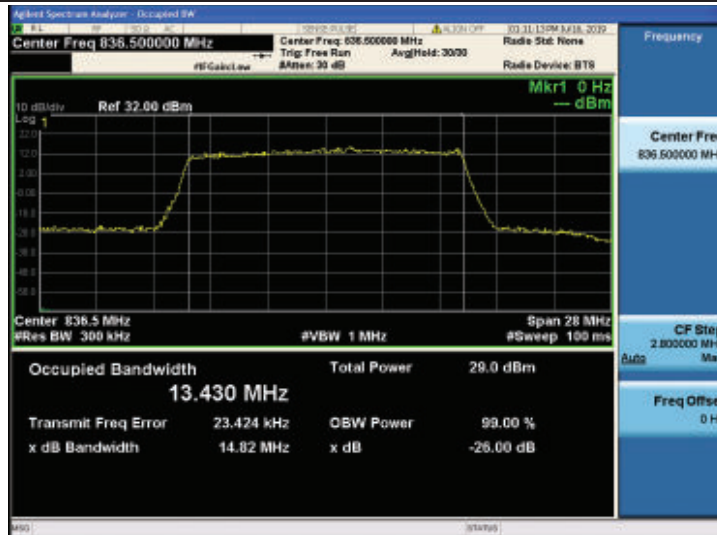
Band26-15MHz-16QAM-26915-75RB#0-13.430
