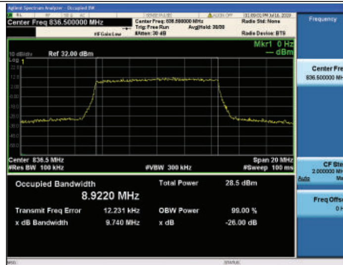
Band26-10MHz-16QAM-26915-50RB#0
