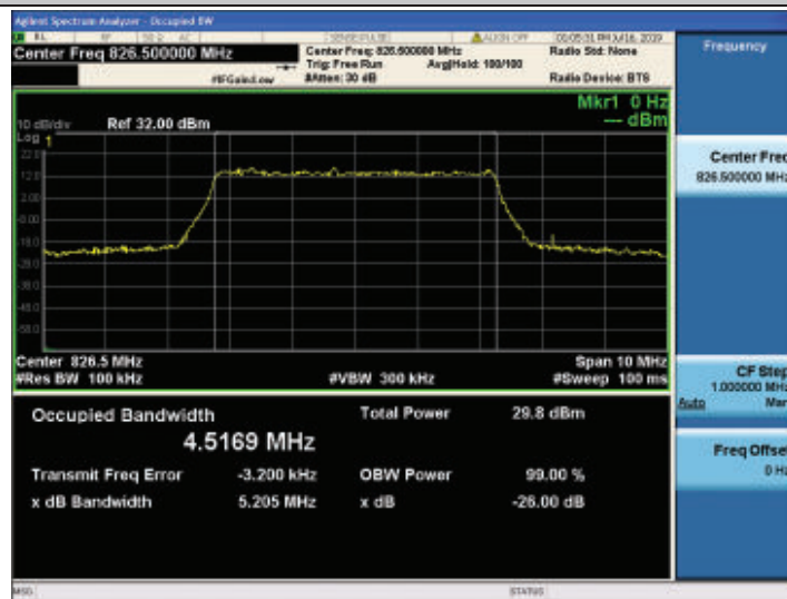
Band26-5MHz-QPSK-26815-25RB#0
