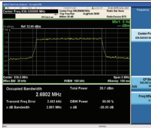
Band26-3MHz-QPSK-26915-15RB#0
