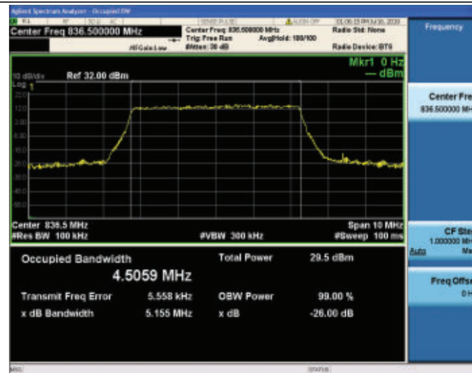
Band26-5MHz-QPSK-26915-25RB#0
