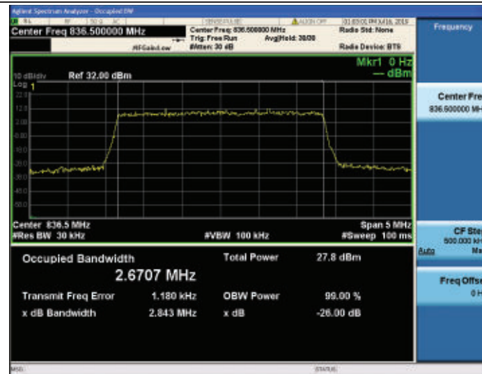
Band26-3MHz-16QAM-26915-15RB#0
