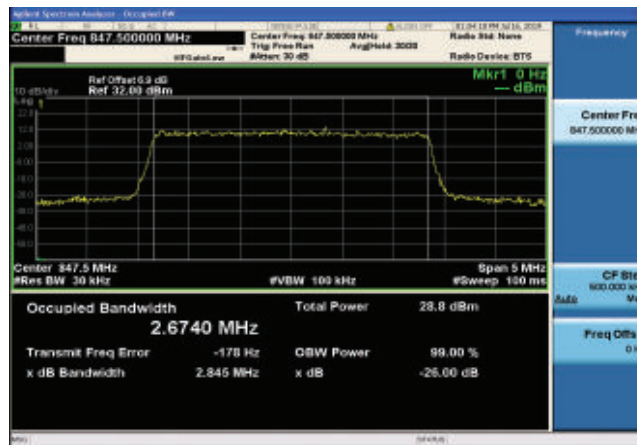
Band26-3MHz-QPSK-27025-15RB#0
