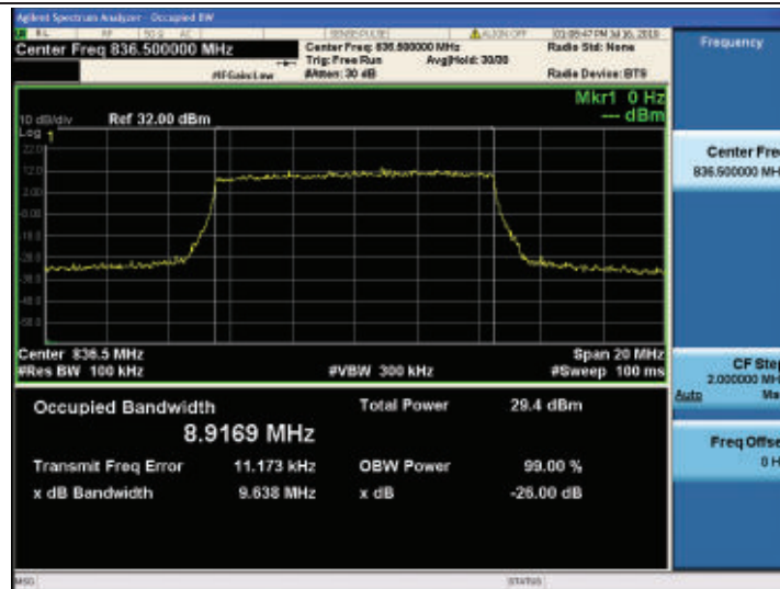
Band26-10MHz-QPSK-26915-50RB#0
