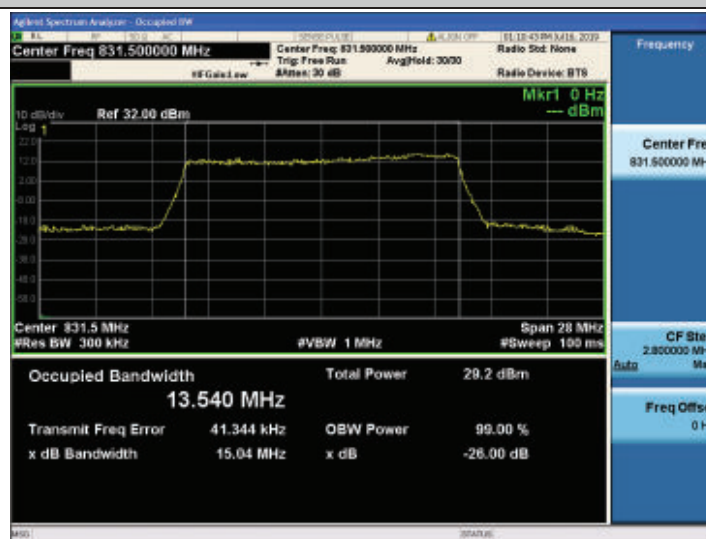
Band26-15MHz-16QAM-26865-75RB#0
