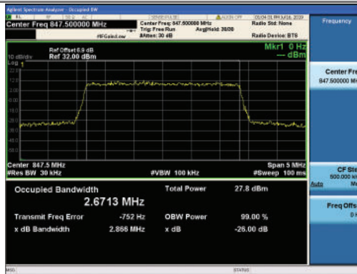
Band26-3MHz-16QAM-27025-15RB#0
