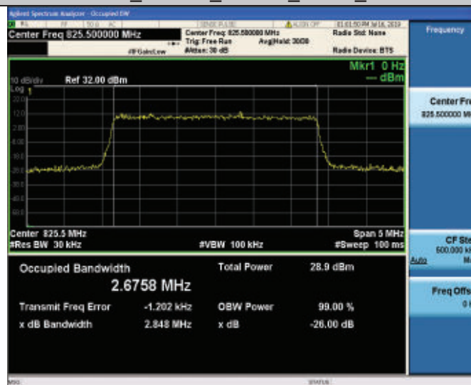
Band26-3MHz-QPSK-26805-15RB#0
