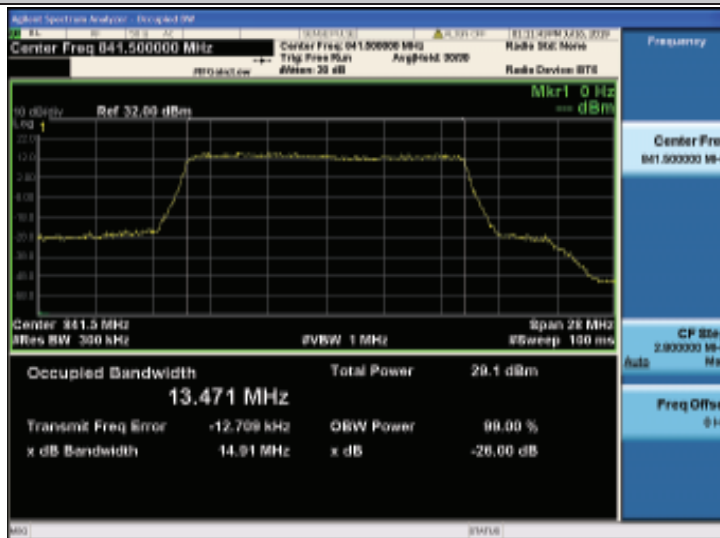
Band26-15MHz-16QAM-26965-75RB#0
