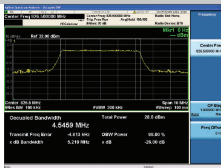
Band26-5MHz-16QAM-26815-25RB#0
