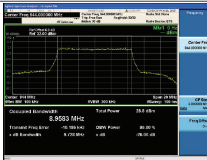
Band26-10MHz-16QAM-26990-50RB#0
