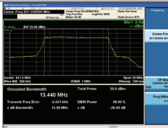
Band26-15MHz-QPSK-26965-75RB#0
