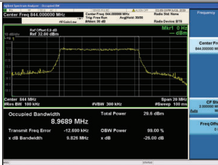
Band26-10MHz-QPSK-26990-50RB#0
