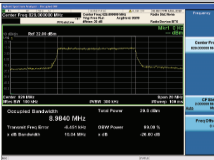
Band26-10MHz-QPSK-26840-50RB#0
