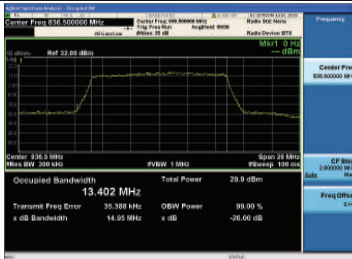
Band26-15MHz-QPSK-26915-75RB#0
