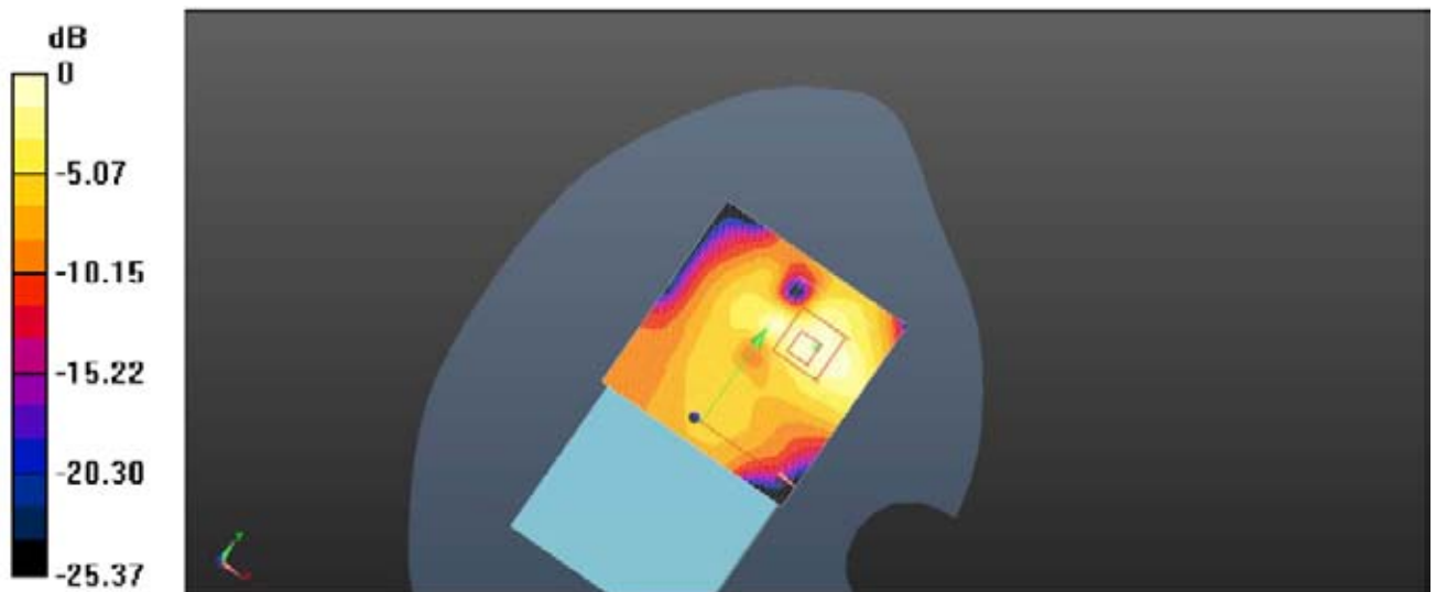
Plot 22: Body Rear Side (GSM1900 Speech With Headset Middle Channel)
