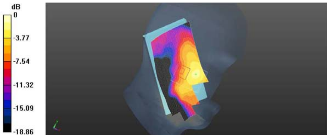
Plot 2: Left Head Tilt (GSM850 Middle Channel)
