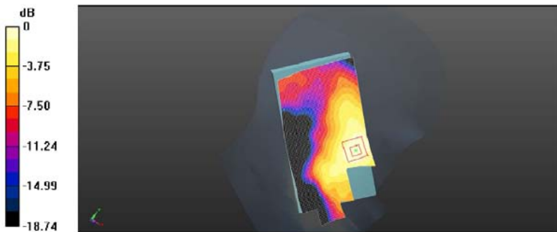
Plot 13: Left Head Tilt (GSM1900 Middle Channel)
