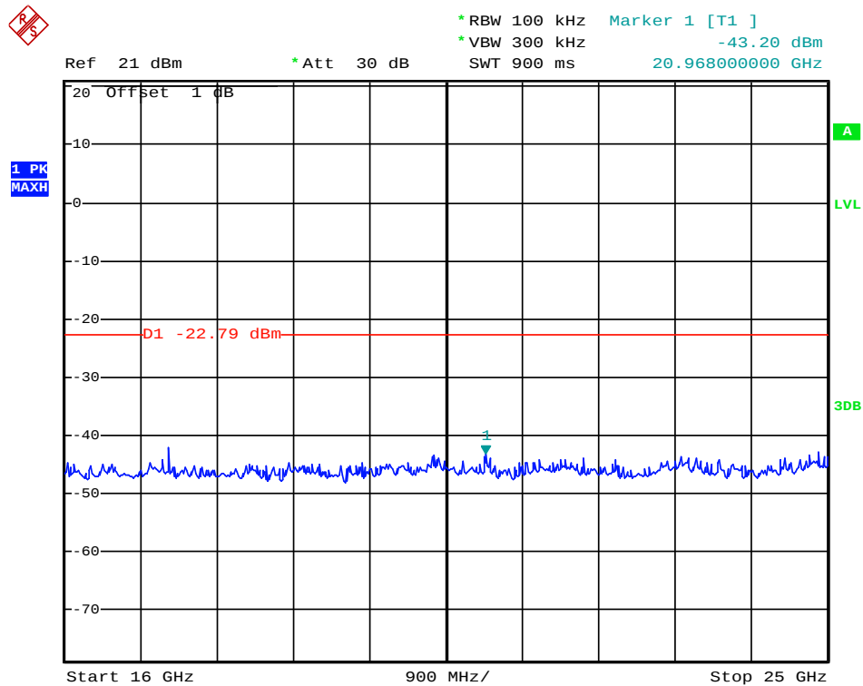
(Plot 4.6.1 B3: Channel 19: 2440MHz @ GFSK)
