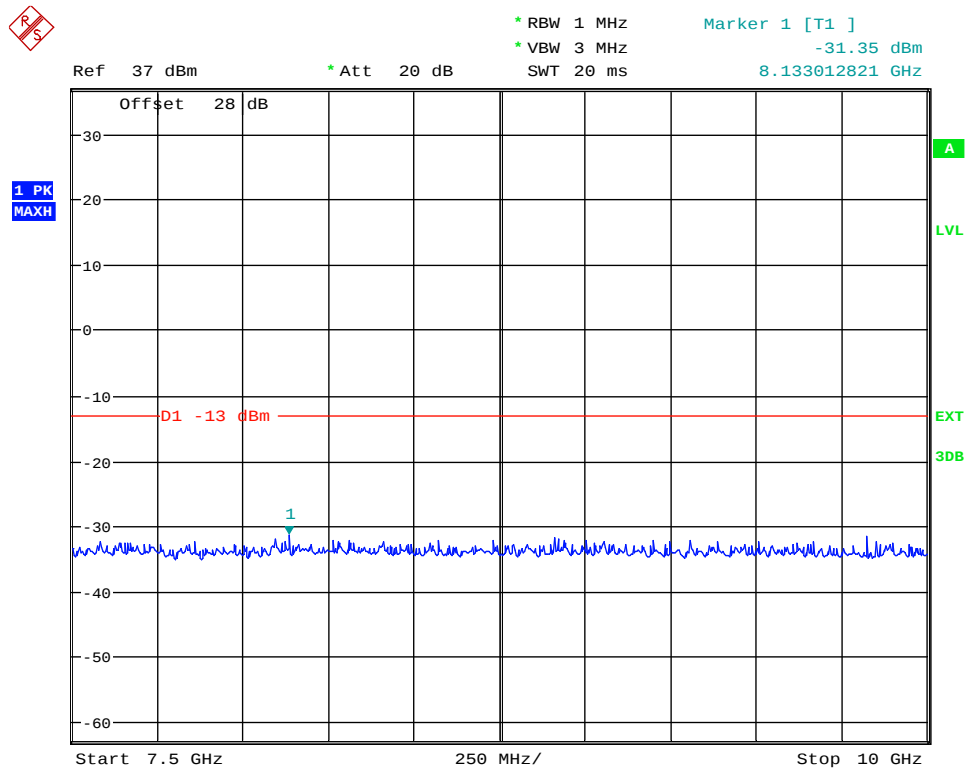
(Plot 4.7.2 A3: Channel 9400: 1880.0MHz @ Traffic WCDMA Band II)
