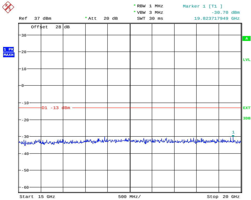
(Plot 4.7.3 A5: Channel 9538: 1907.6MHz @ Traffic WCDMA Band II)
