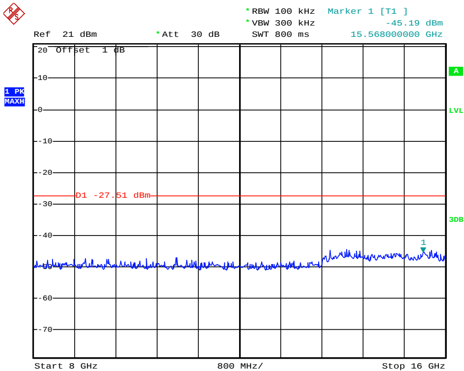
(Plot 4.6.4 C2: Channel 9: 2452MHz @ 802.11n(40MHz))
