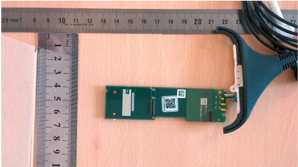
Fig.5 P4TR-AA-ADS HDI2 (bottom view )
