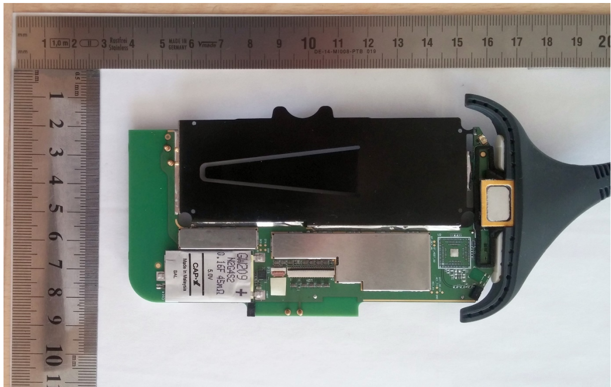
Fig.3 P4TR-AA-ADS HDI1 (top view)
