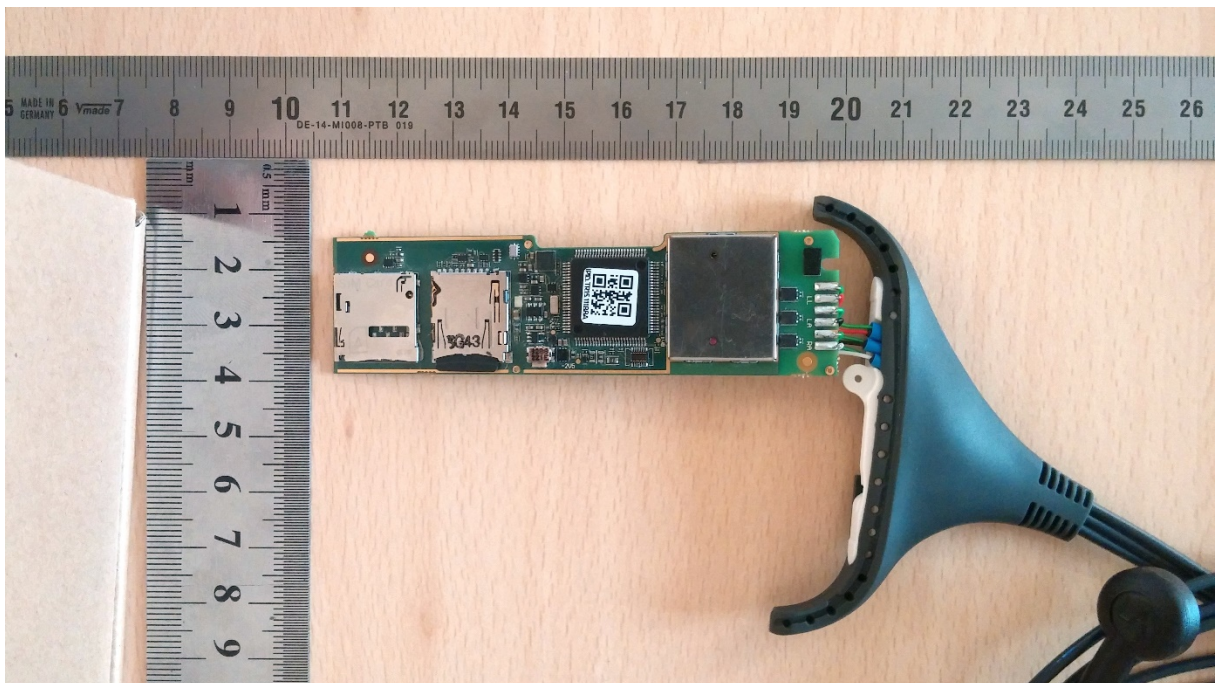
Fig.6 P4TR-AA-ADS HDI2 (top view )
